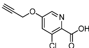
Intermediate 47
