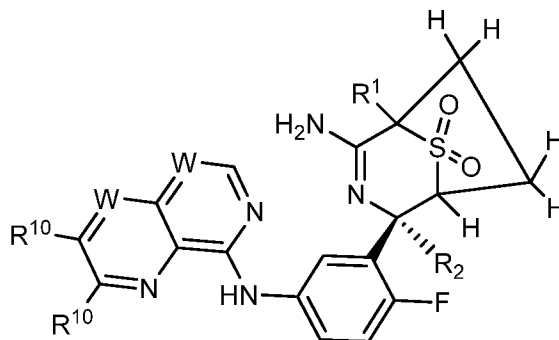
II-A-b
