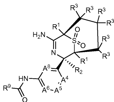
III-A-1
