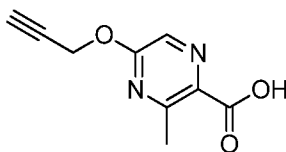
Intermediate 50
