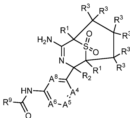
III-A
