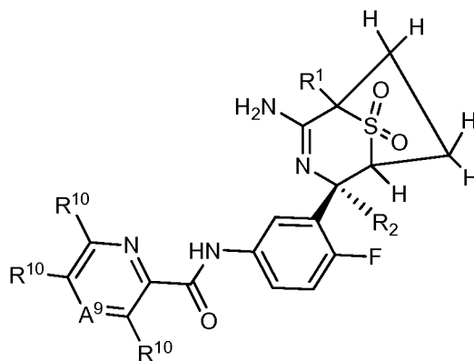
II-A-a
