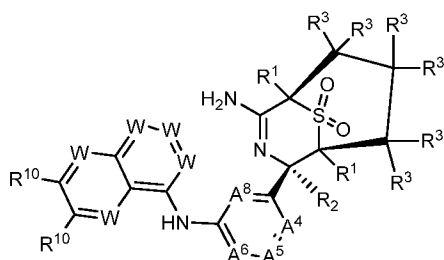
III-B-1 and
