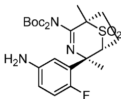
Intermediate 13
