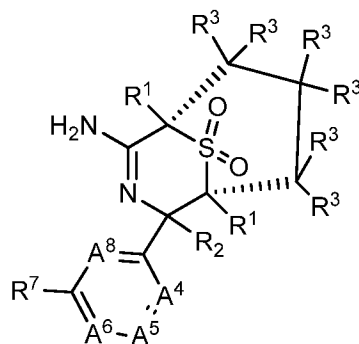
III-C
