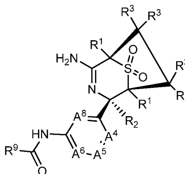
II- C-1-B
