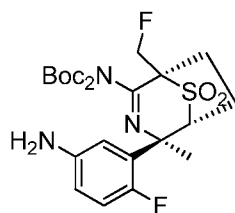
Intermediate 39
