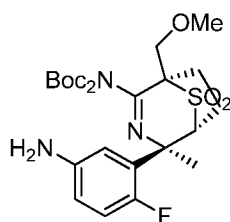
Intermediate 34
