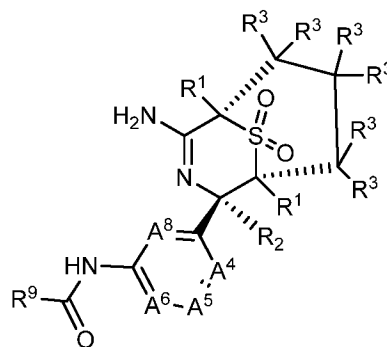
III-A-2
