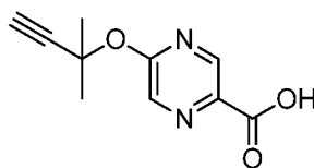
Intermediate 29
