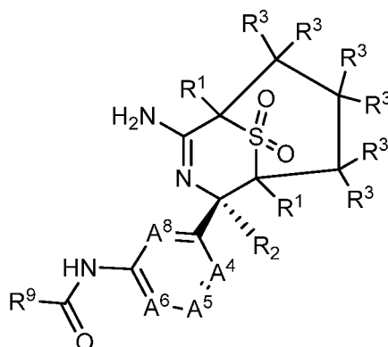
III-A-1
