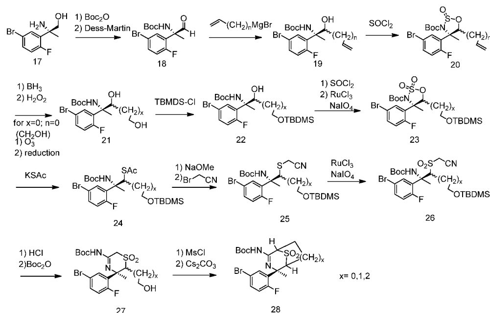
Scheme 2
