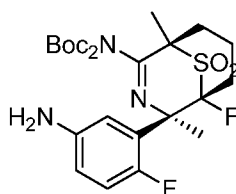
Intermediate 3
