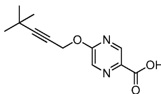
Intermediate 28
