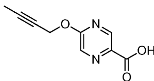
Intermediate 54
