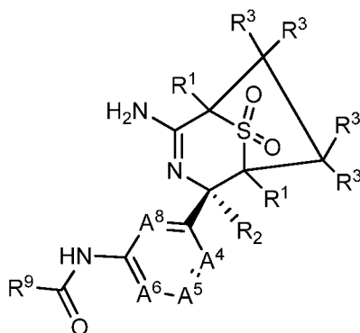
II-C-1
