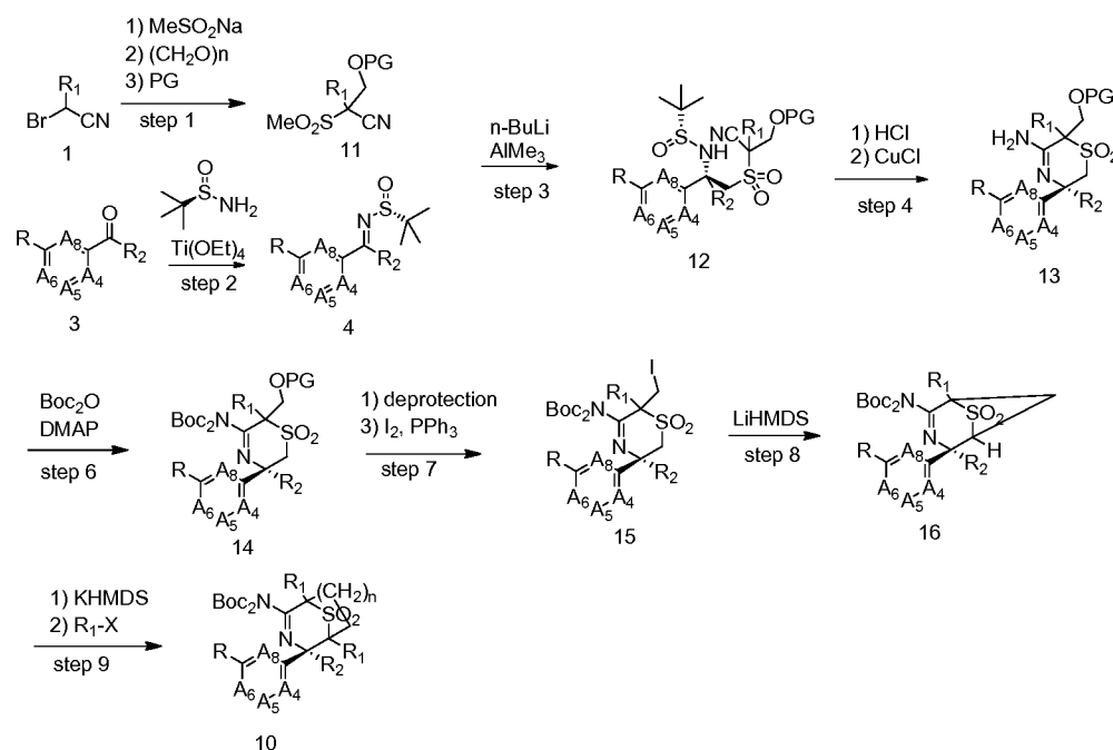
Scheme 1-B
