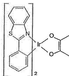
Bt 2 (acac)
