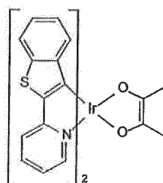
Btp 2 (acac)
