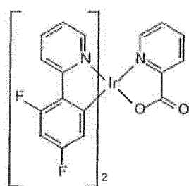
FIr(pic)
