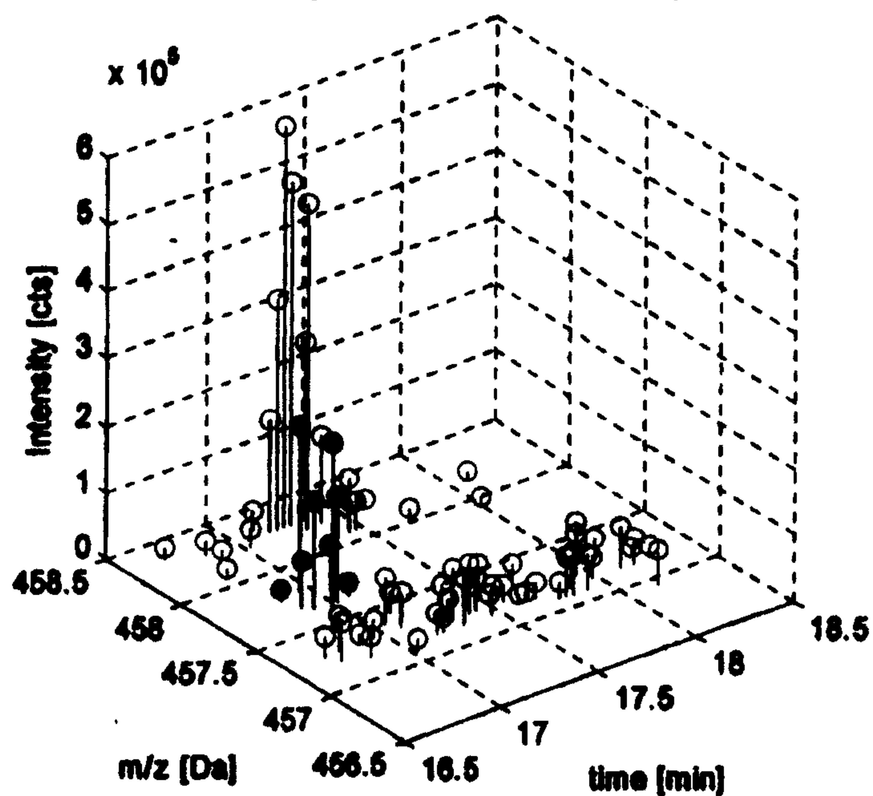
Fig. 21 These data points are identified to be caused by ions of the same type
