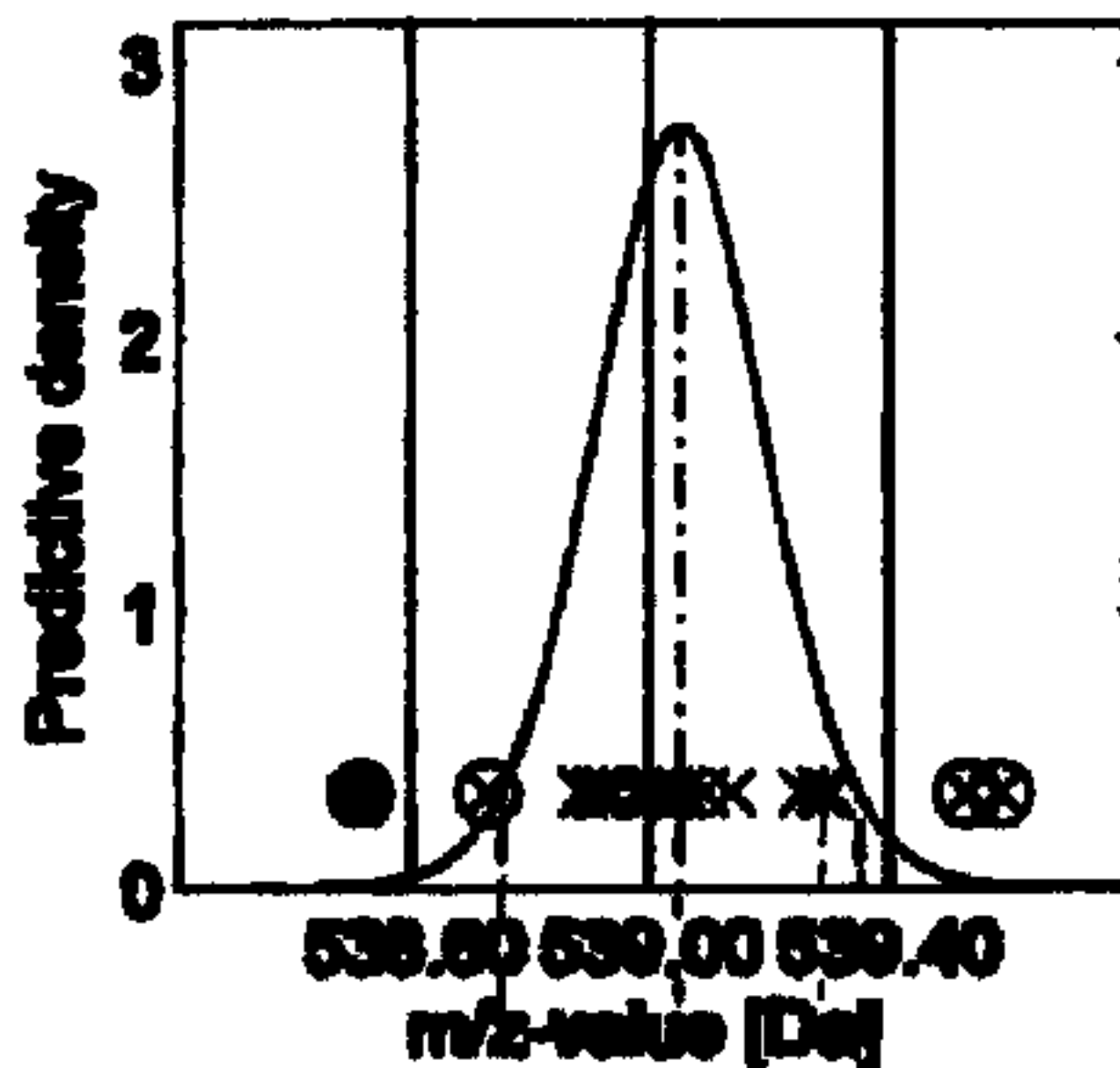
Grouping after 19 observation(s)
