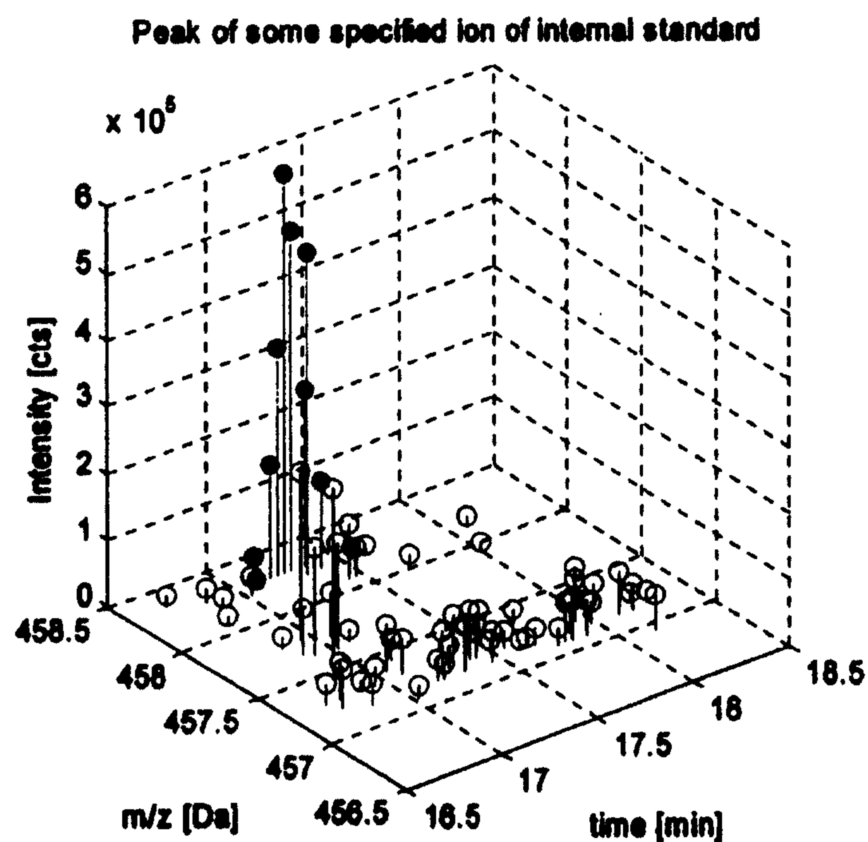
FIG. 18 These data points were identified as being caused by one of the specified ions of the internal standards. Mass error distribution is checked and learnt with these points among others
