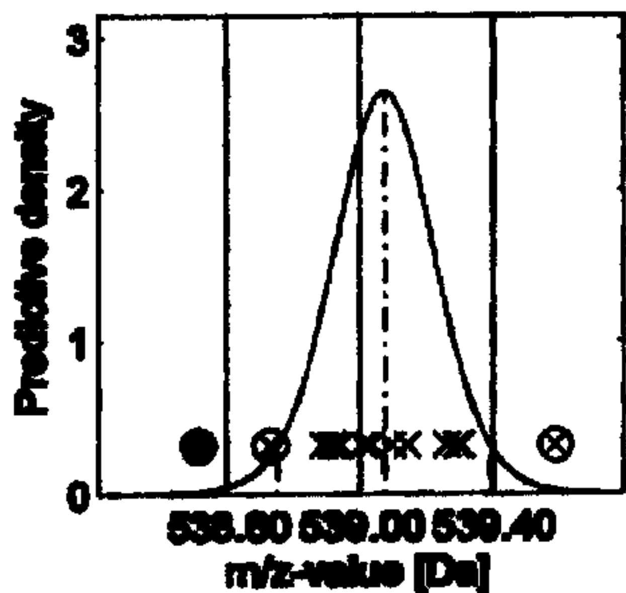
Grouping after 15 observation(s)
