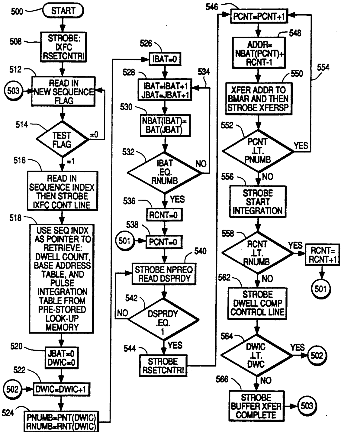
FIG. 3d
