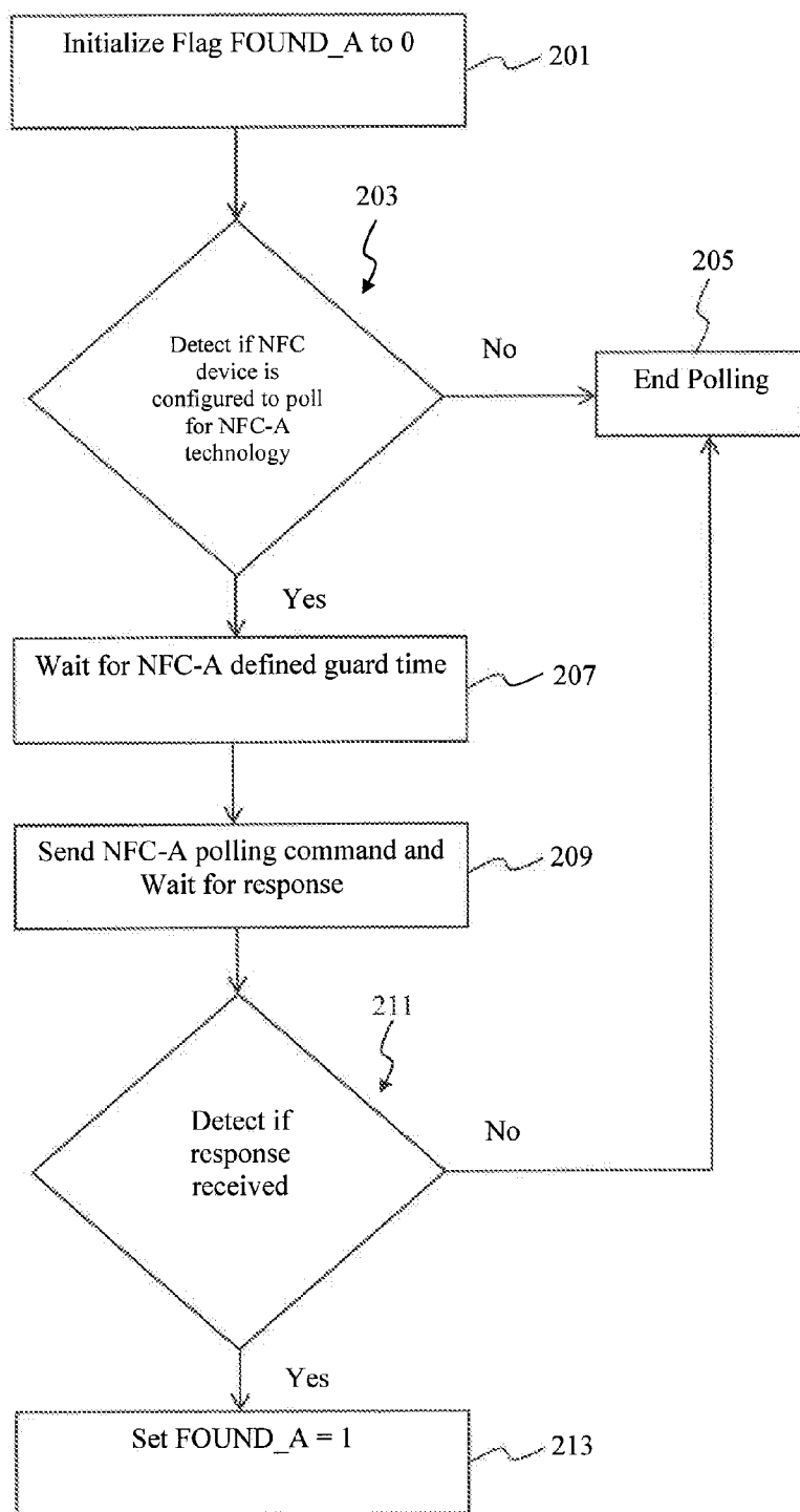
FIG. 2 (Prior Art)
