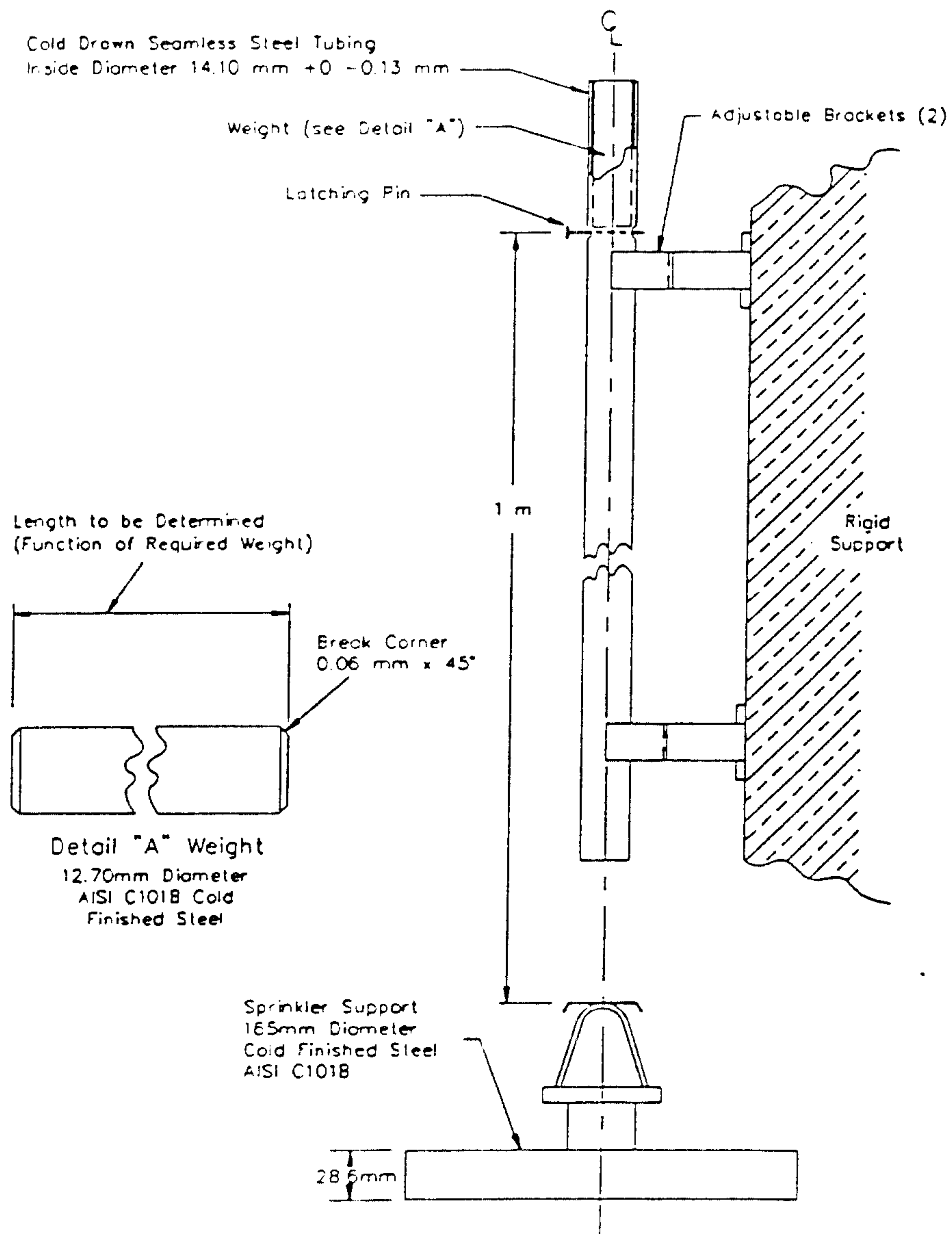
Figure 26.1 Impact test apparatus
