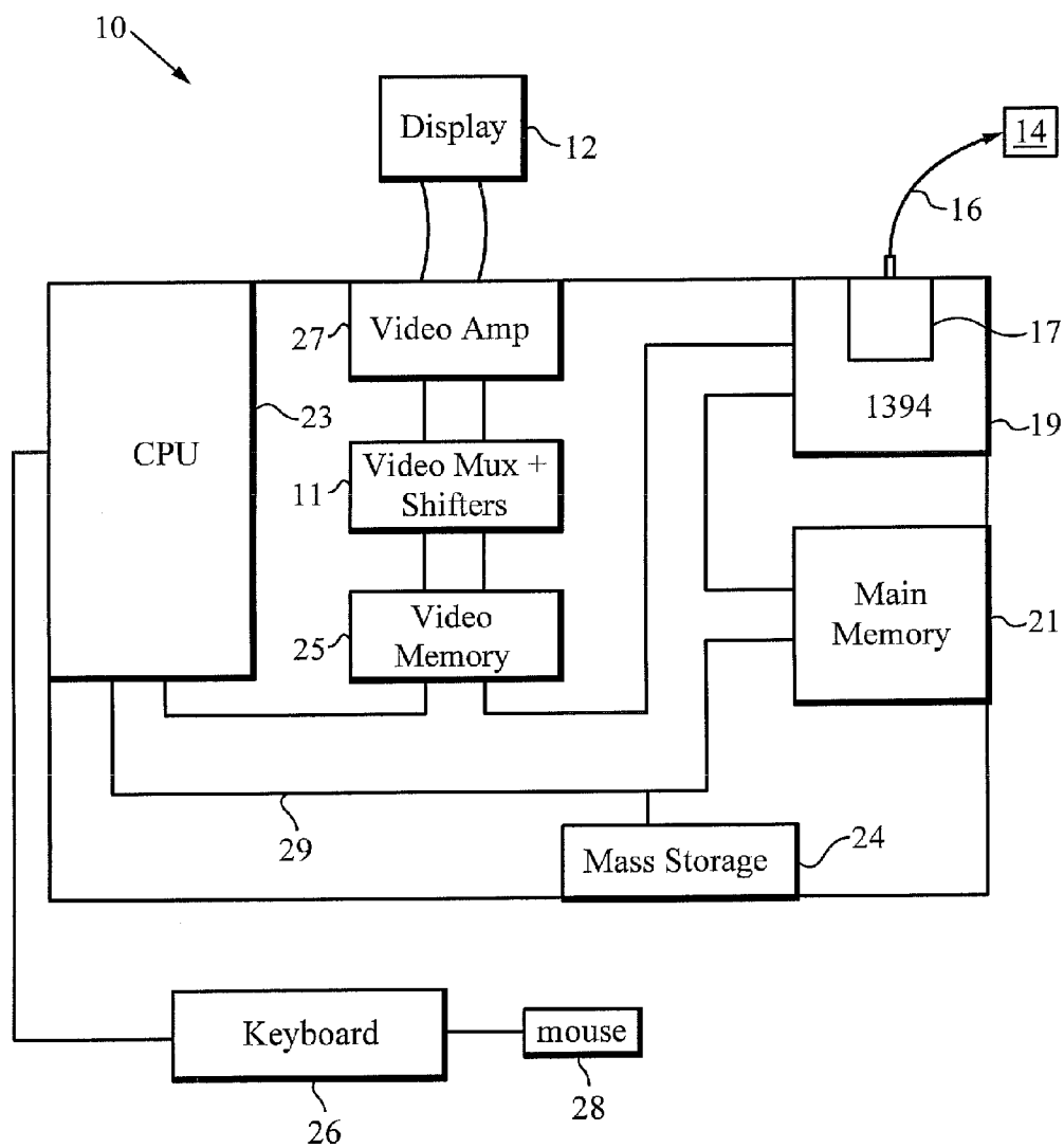
Fig. 2 (PRIOR ART)
