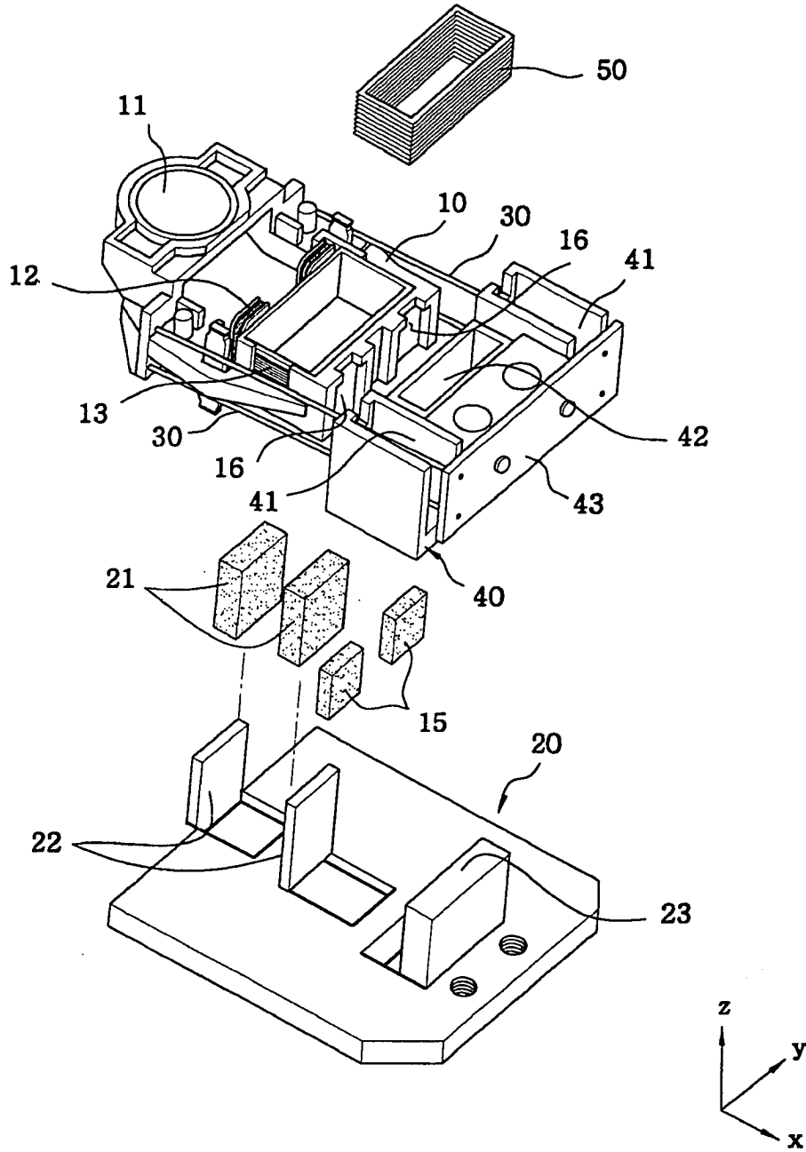
Fig.2 Related Art
