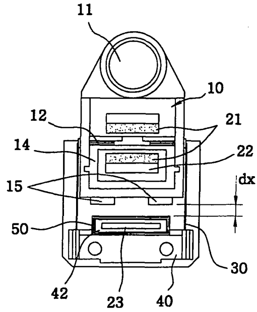
Fig.3 Related Art
