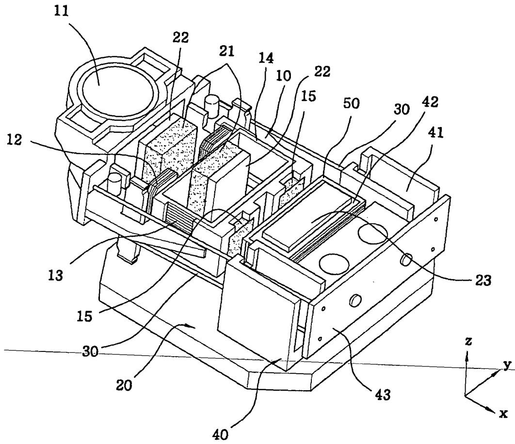
Fig.1 Related Art
