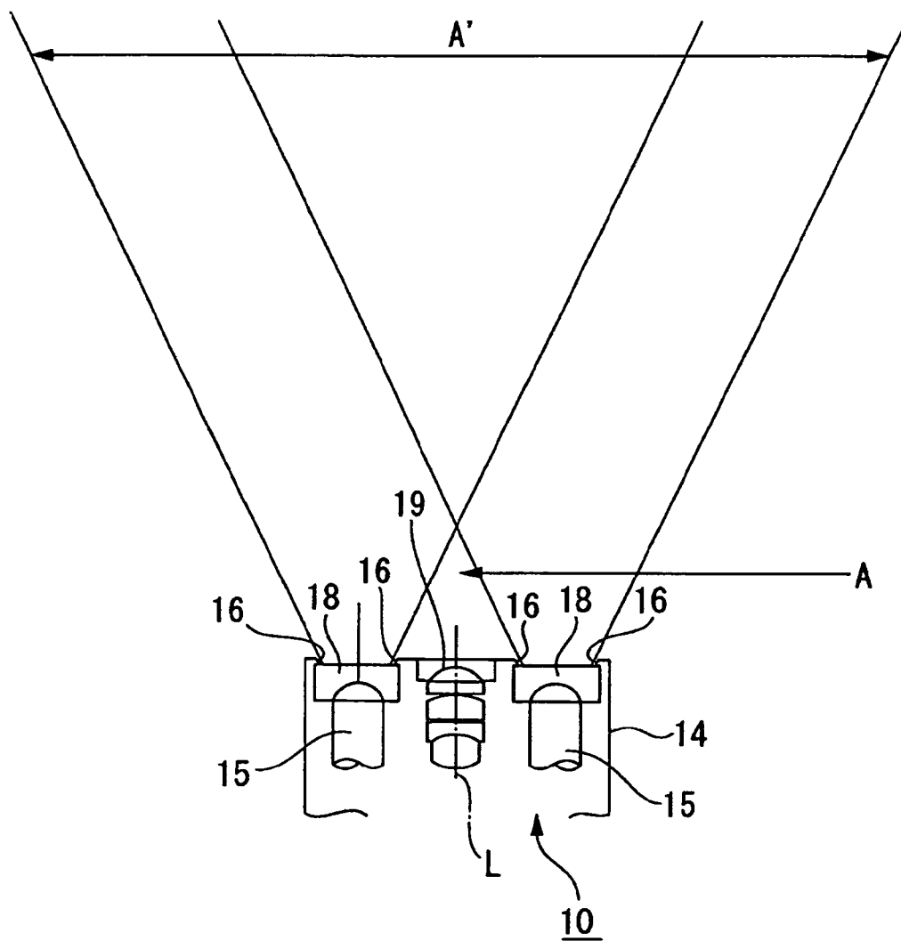
FIG. 10 Prior Art
