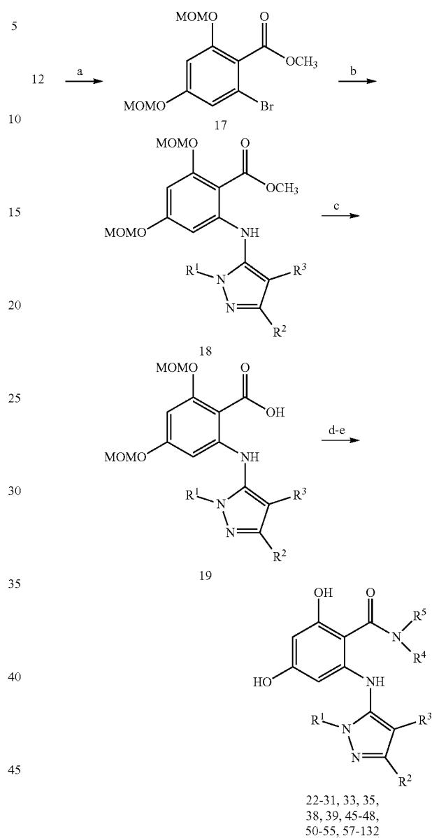
Scheme C. Second-generation synthetic route to aminopyrazole resorcyate amides
