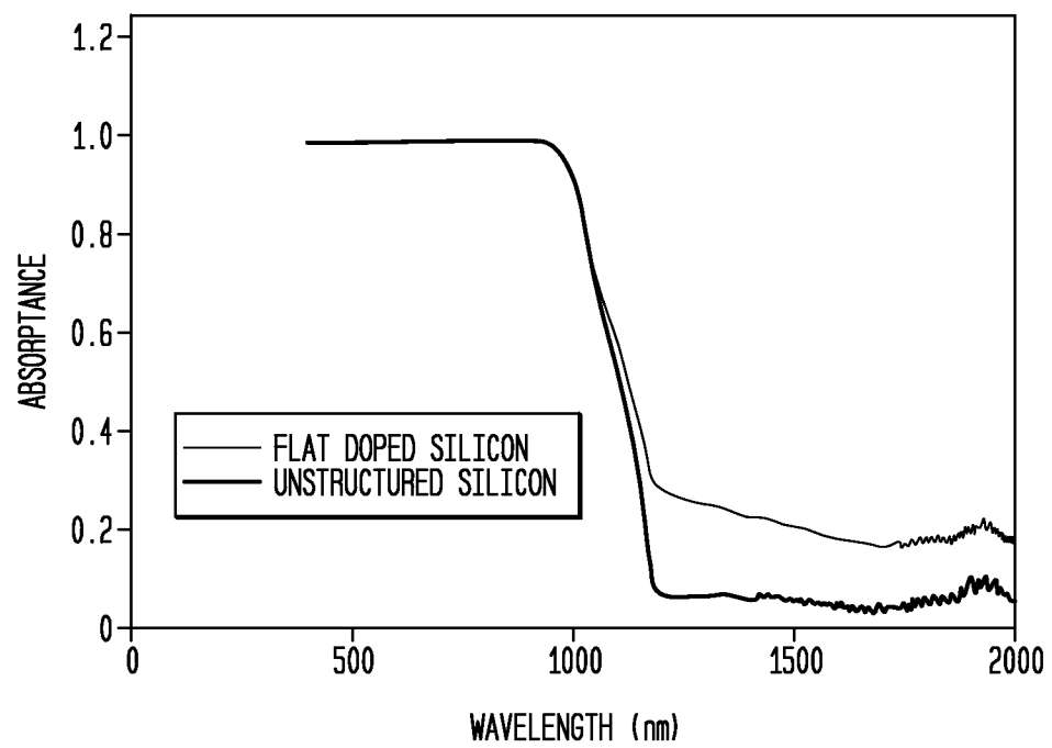
FIG. 8 NORMALIZED ABSORPTANCE
