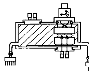
FIG. 8I: FINE ALIGNMENT
