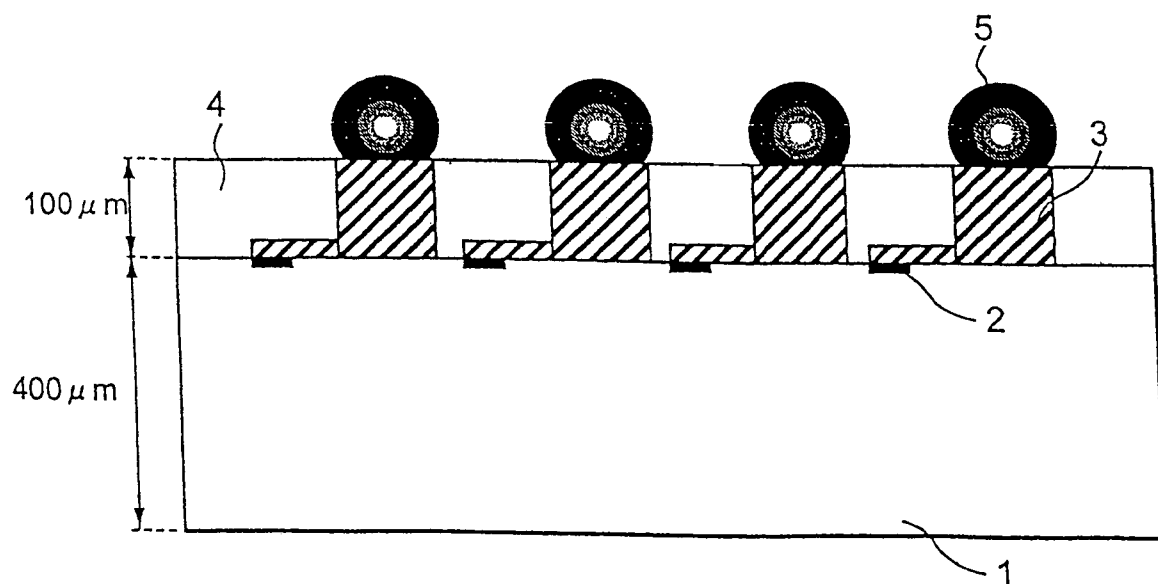
FIG. 9 PRIOR ART
