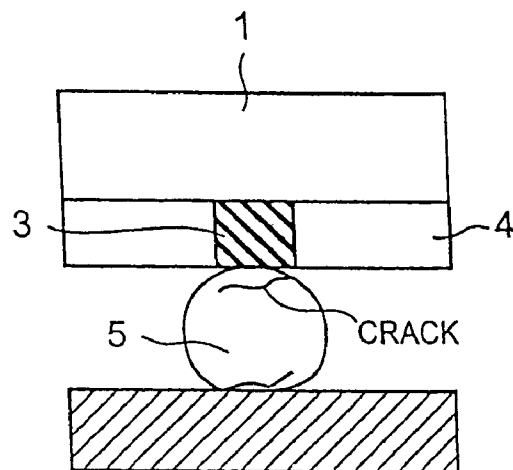
FIG.11 PRIOR ART
