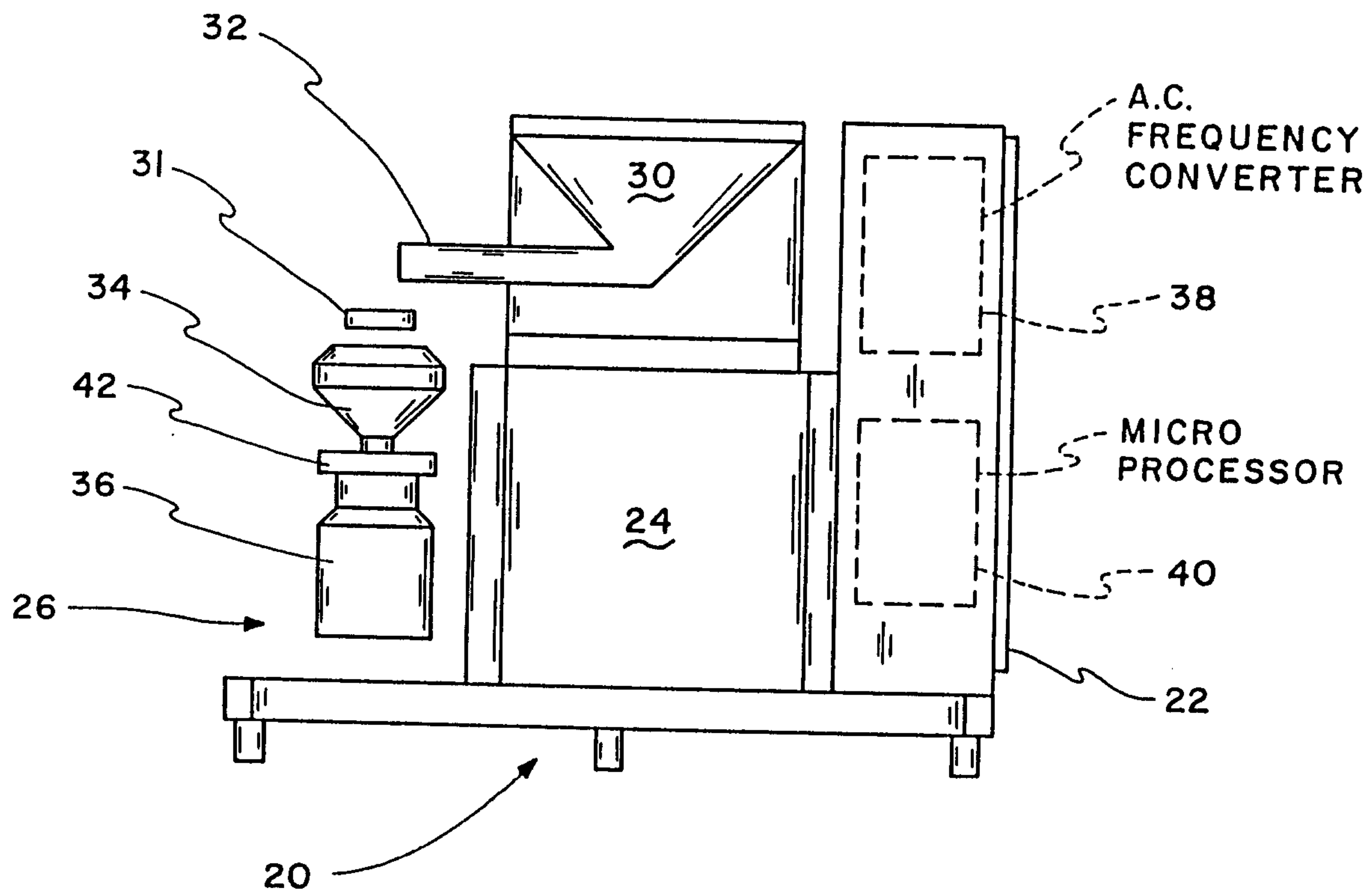
FIG. 1 (PRIOR ART)
