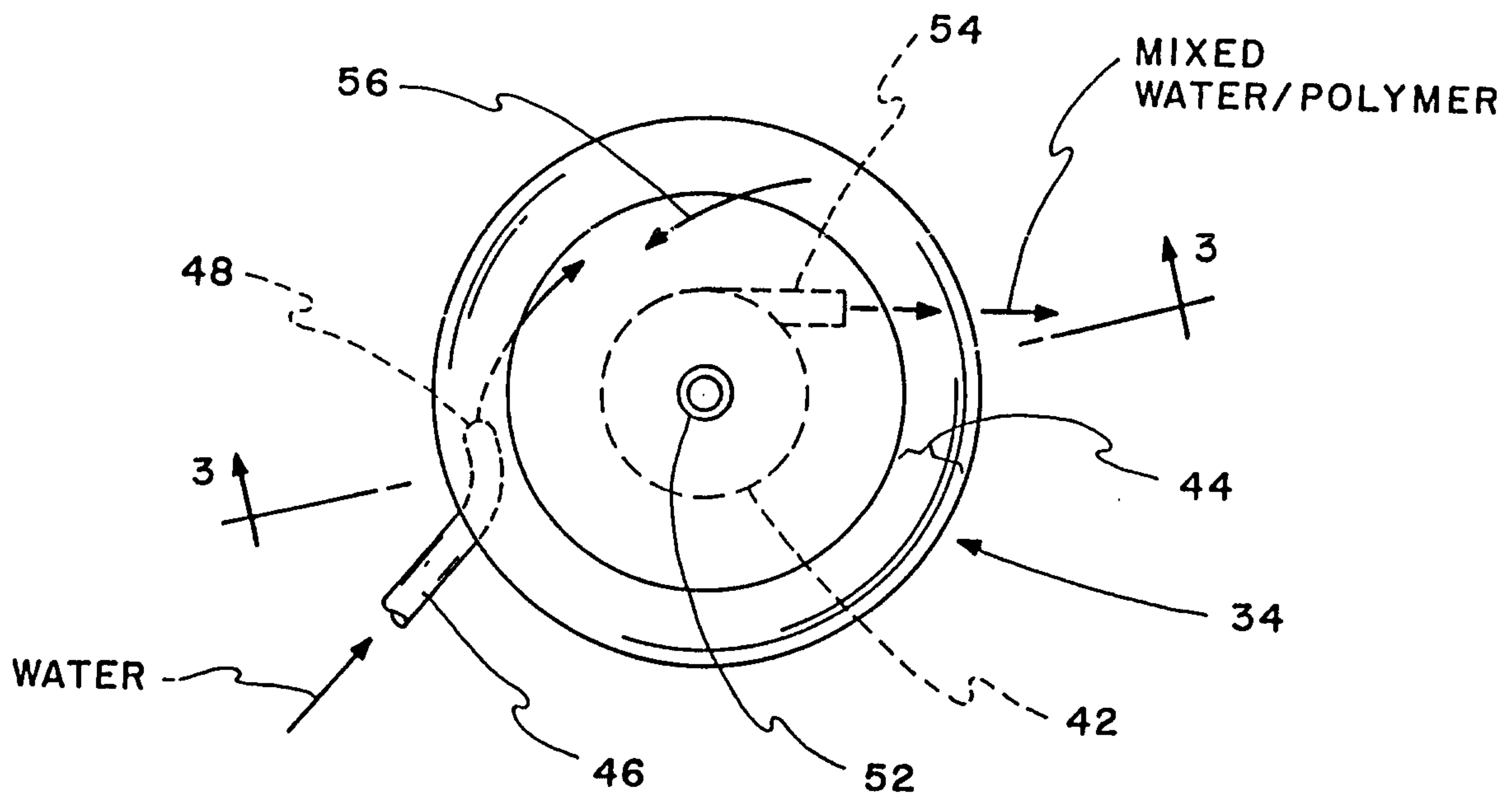
FIG. 2 (PRIOR ART)
