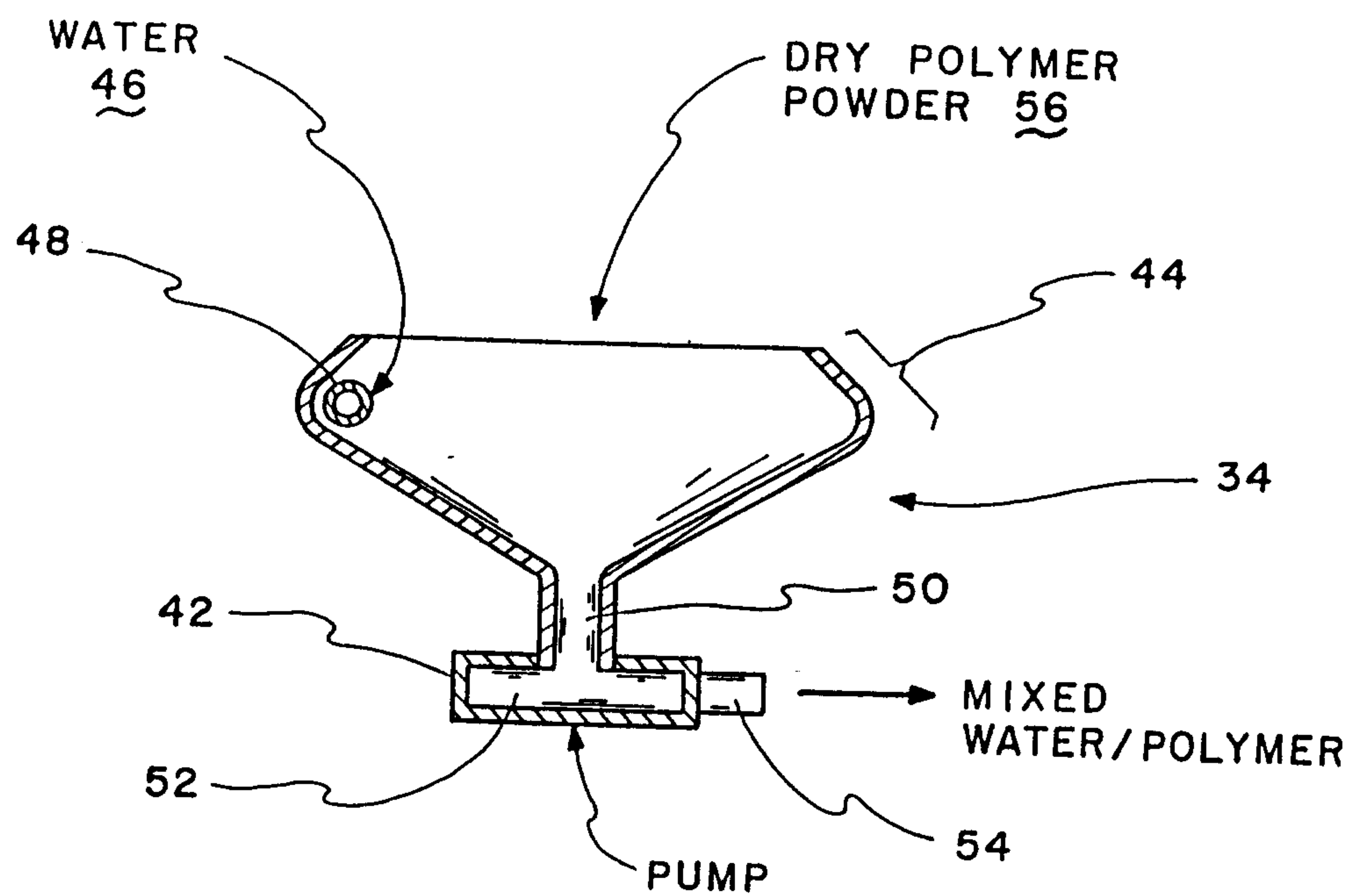
FIG. 3 (PRIOR ART)
