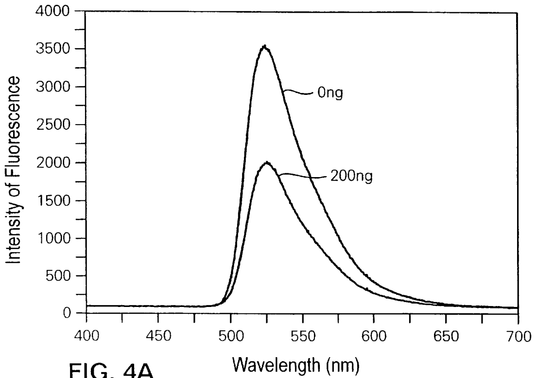
Wildtype Sp1:wildtype JD11F/12F binding
