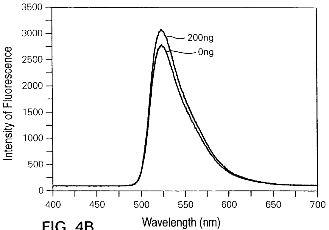
Wildtype Sp1:mutant JD13F/14F binding
