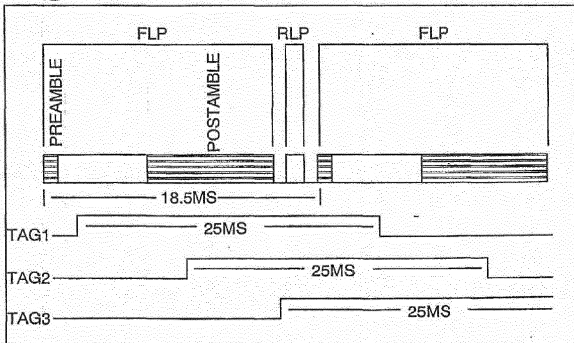
TAG RECEIVER WAKEUP
