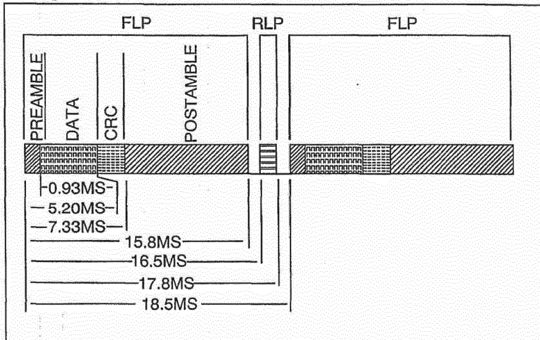
TIMING DIAGRAM WITH PREAMBLE, CRC, POSTAMBLE
