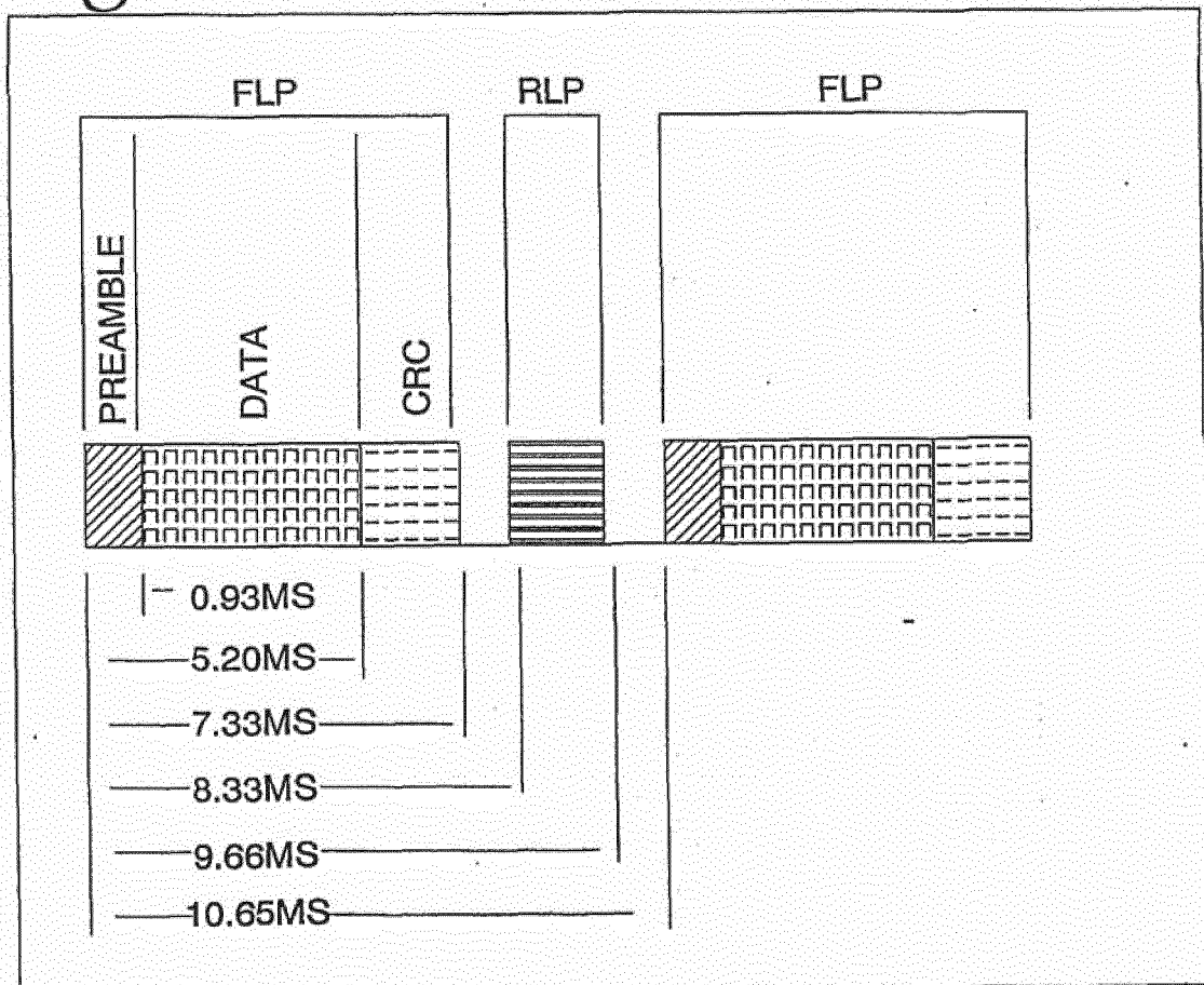
TIMING DIAGRAM WITH PREAMBLE & CRC
