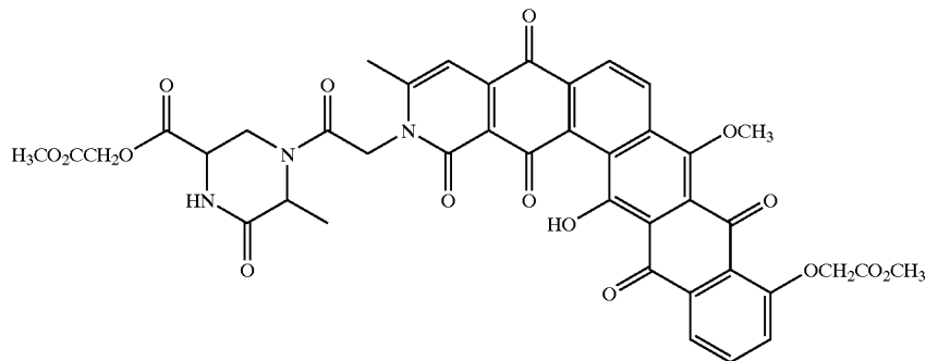
P175A ETHER B
