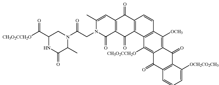
P175A ETHER C
