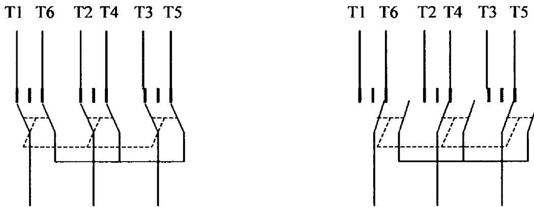
Speed switch: at low speed position
