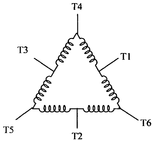
Winding of a multi-speed motor
