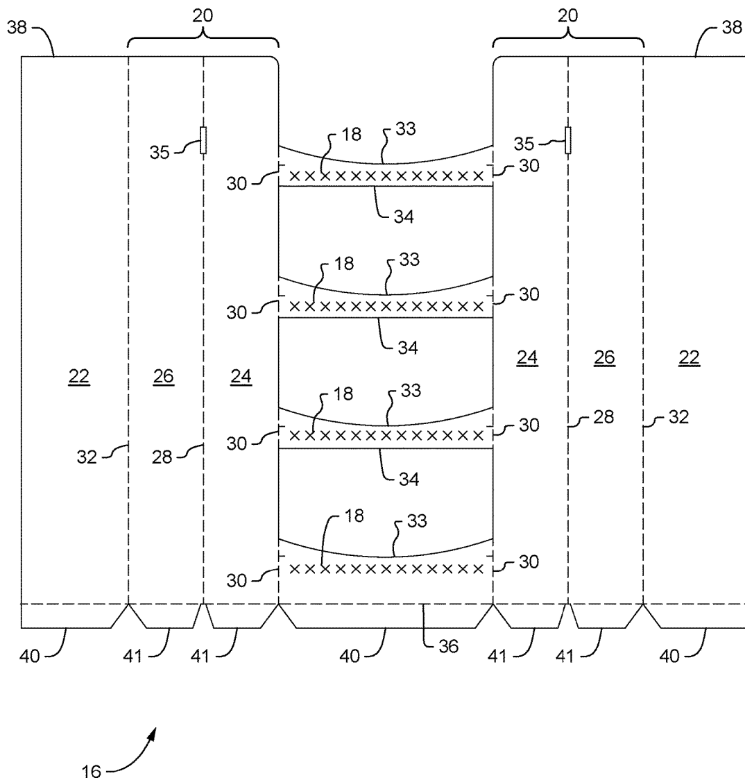
FIG. 2 (Hutch Body Blank)
