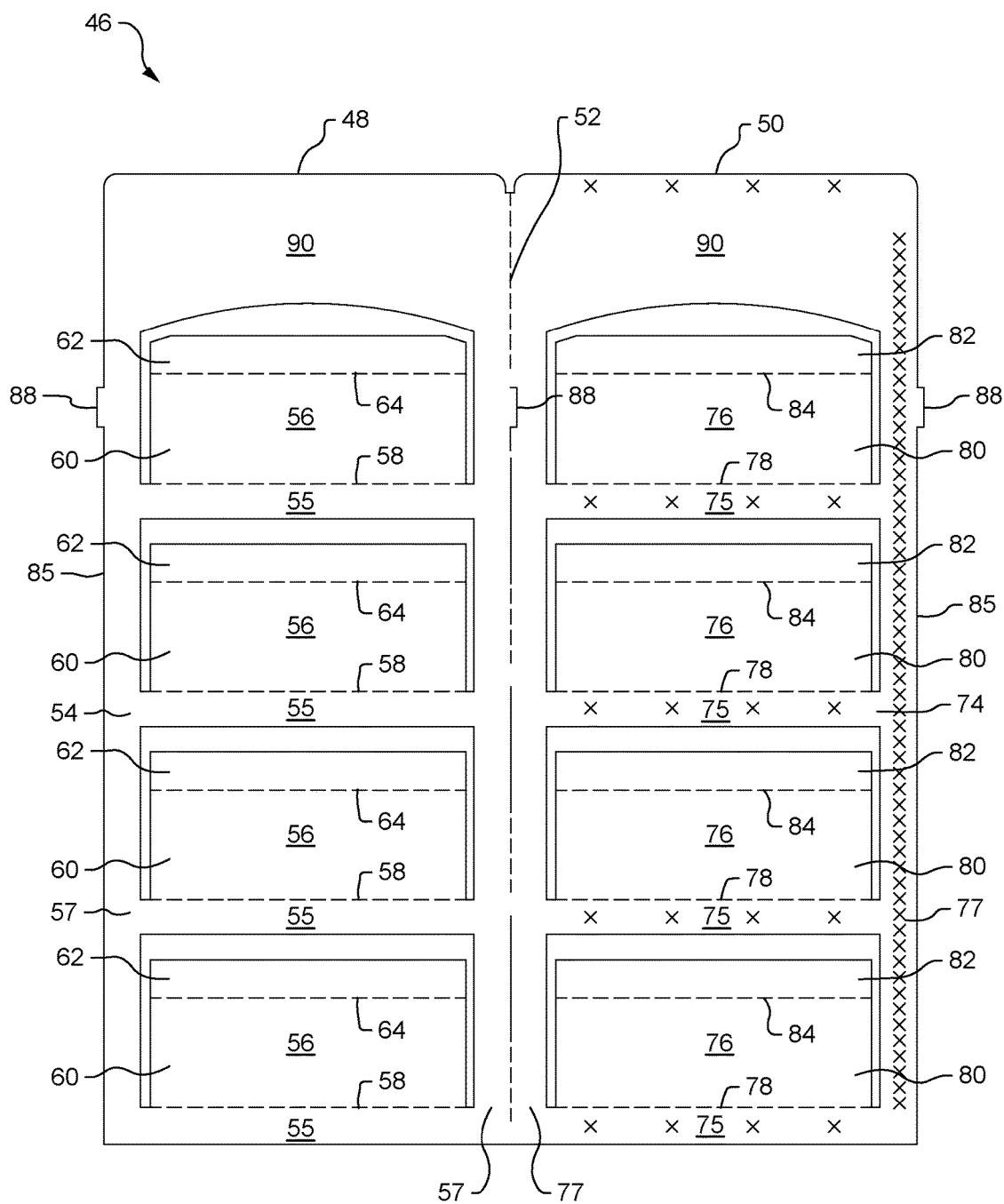
FIG. 3 (Hutch Spine Blank)
