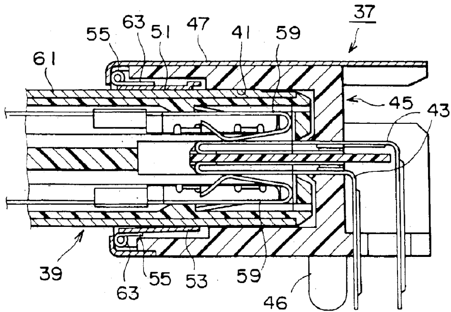
FIG. 3 PRIOR ART
