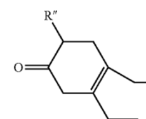
5 substituted cyclohexen- 4-one
