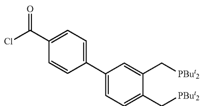
1,2-bis(di-tert-butyl(phosphinomethyl))-4-(4'-chlorocarbonyl-phenyl)benzene
