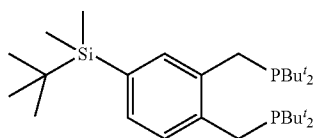
1,2-bis(di-tert-butyl(phosphino-methyl))-4-trimethylsilyl benzene
