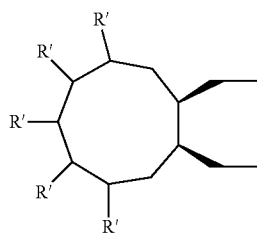
4, 5, 6, 7 and/or 8 substituted cyclononyl
