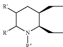
5 and/or 6 substituted piperidines
