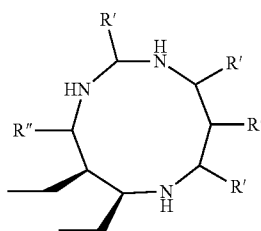
Substituted 1, 5, 9 triazacyclodecane
