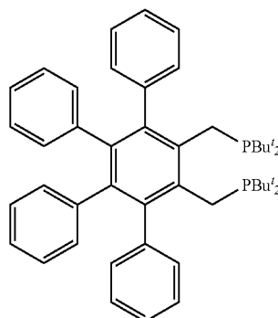
1,2-bis(di-tert-butyl(phosphino-methyl))-3,4,5,6-tetraphenyl benzene
