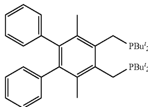
1,2-bis(di-tert-butyl(phosphino-methyl))-3,6-dimethyl-4,5-diphenyl benzene
