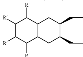
2, 3, 4 and/or 5 substituted decahydronaphthalene
