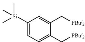
1,2-bis(di-tert-butyl(phosphino-methyl))-4-trimethylsilyl benzene
