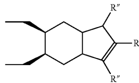
Substituted 3a, 4, 5, 6, 7, 7a-hexahydro-1H-indene
