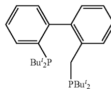
2-(di-tert-butylphosphino-methyl)-2'-(di-tert-butylphosphino)-biphenylene
