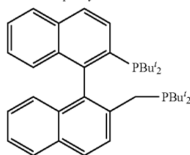
2-(di-tert-butylphosphinomethyl)-2'-(di-tert-butylphosphino)-binaphthylene
