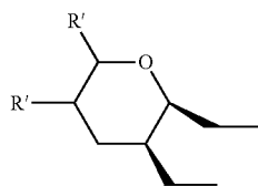
substituted tetrahydropyran
