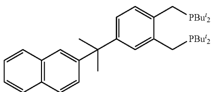
1,2-bis(di-tert-butyl(phosphinomethyl))-4-(2'-naphthylprop-2'-yl)benzene
