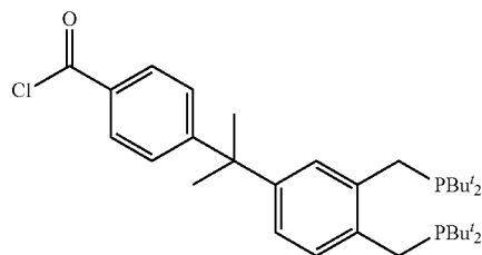
4-(1-(3,4-Bis-[(di-tert-butyl-phosphanyl)-methyl]-phenyl)-1-methyl-benzoyl) benzoyl chloride
