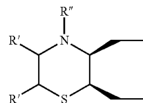
1, 2, 3 substituted thiomorpholine
