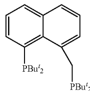
1-(di-tert-butylphosphino)-8-di-tertbutylphosphino-methyl-naphthalene
