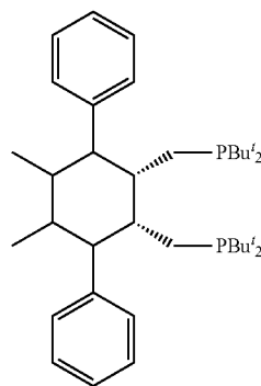
cis-1,2-bis(di-tert-butylphosphinomethyl)-3,6-diphenyl-4,5-dimethyl-cyclohexane,
