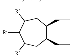
4, 5 and/or 6 substituted cycloheptyl
