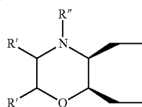
5 and/or 6 substituted morpholines
