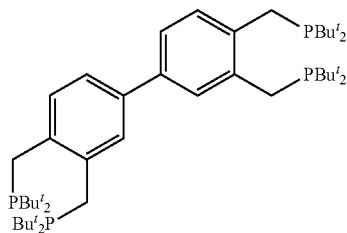
1,2-bis(di-tert-butyl(phosphinomethyl))-4-(3',4'-bis(di-tert-butyl(phosphinomethyl))phenyl)benzene
