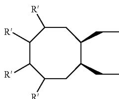
4, 5, 6 and/or 7 substituted cyclooctyl
