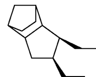
Octahydro-4, 7 methano-indene
