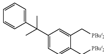
1,2-bis(di-tert-butyl(phosphino-methyl))-4-(2'-phenylprop-2'-yl) benzene
