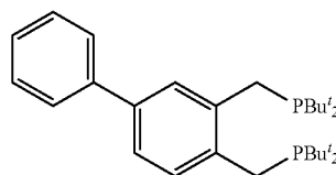
1,2-bis(di-tert-butyl(phosphino-methyl))-4-phenyl benzene
