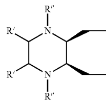
1, 2, 3, 4 substituted piperazine
