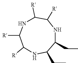
Substituted 1, 4, 7 triazacyclononane
