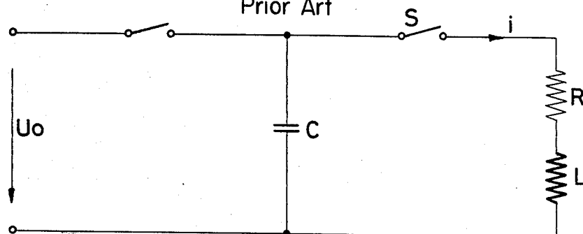
Fig.2 Prior Art
