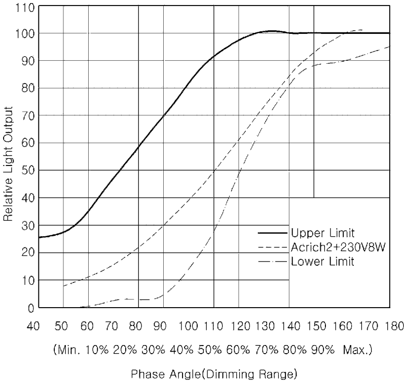
Dimming Light Output Curve
