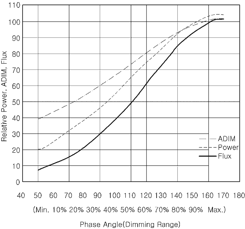
Dimming ADIM, Power, Flux Curve
