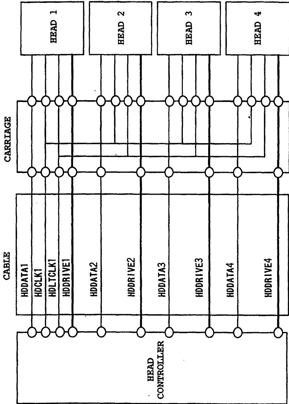
SECOND CONVENTIONAL CONNECTION METHOD
