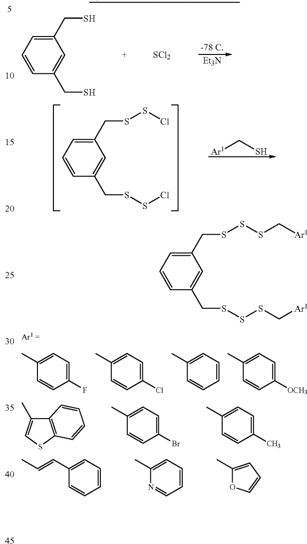
Scheme 5. Synthesis of bis(trisulfide) derivatives
