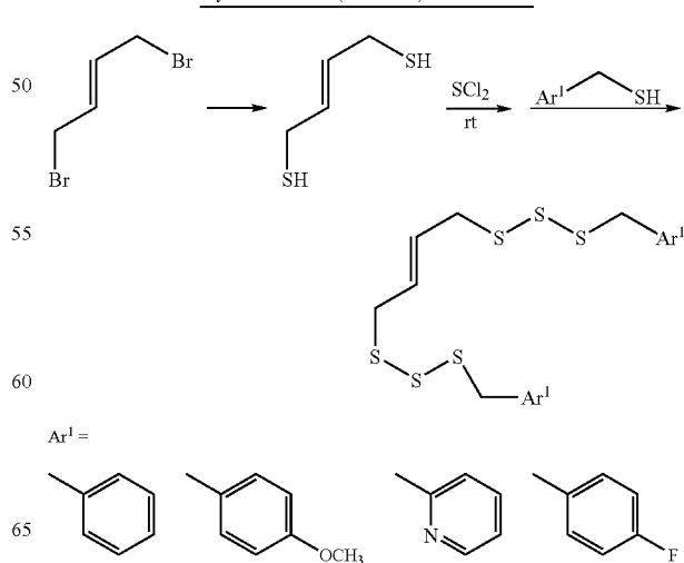
Scheme 5. Synthesis of bis(trisulfide) derivatives
