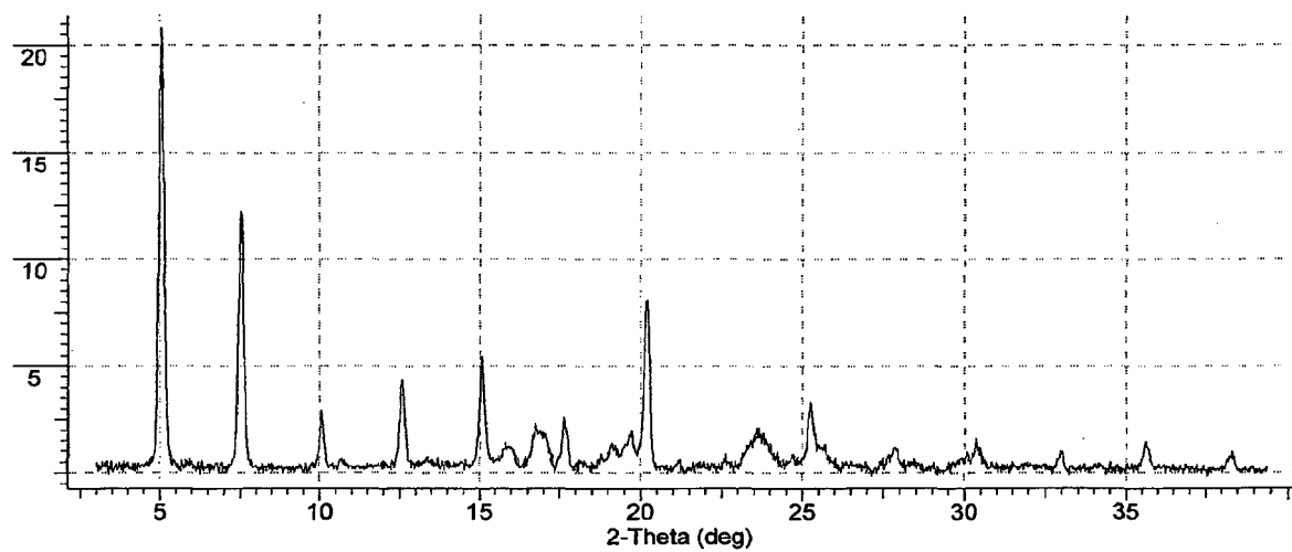
Figure 2.4: X-ray Powder Diffraction Pattern (PXRD) of Modification D
