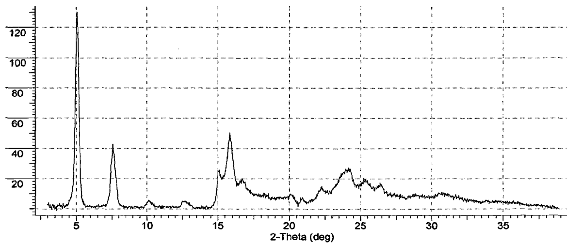
Figure 2.12: X-ray Powder Diffraction Pattern (PXRD) of Modification L
