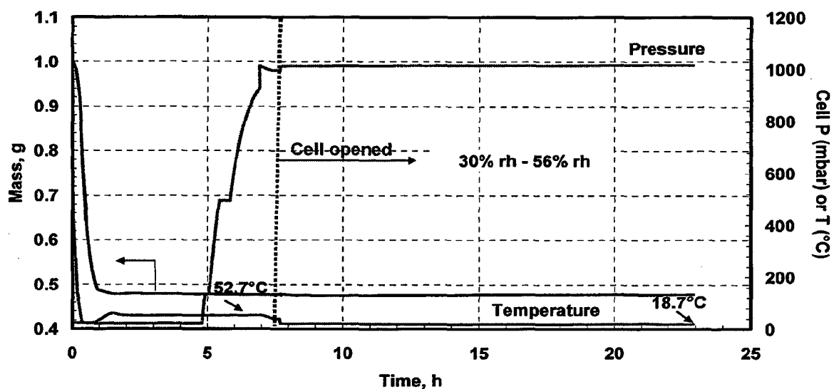
Figure 4: Vacuum thermogravimetric analysis (VTGA) experiment showing the effect of RH (relative humidity) on sample mass of wet cake of Modification C (in acetonitrile and water 8% wt. at 20°C for ~19 hrs.)
