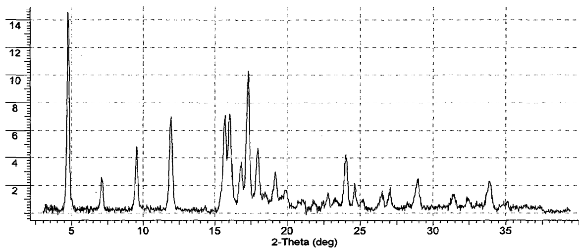
Figure 2.6. X-ray Powder Diffraction Pattern (PXRD) of Modification F
