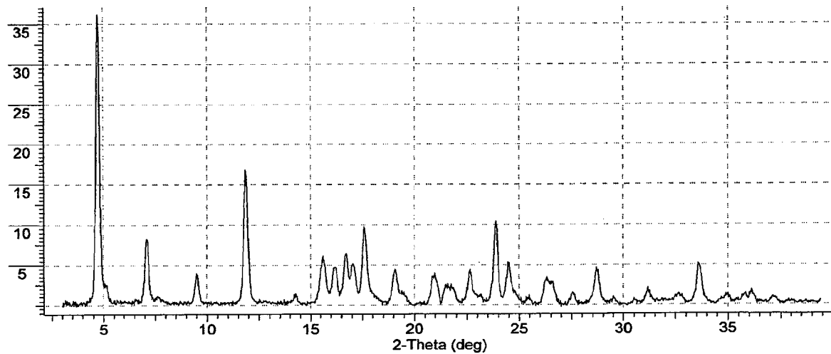
Figure 2.8: X-ray Powder Diffraction Pattern (PXRD) of Modification H
