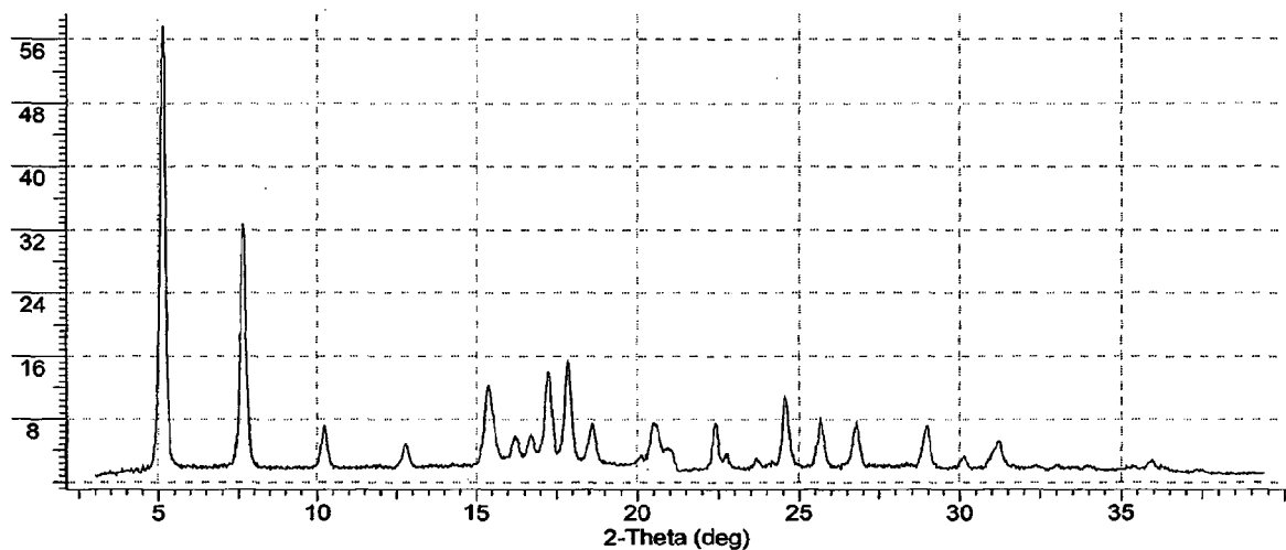
Figure 2.1 X-ray Powder Diffraction Pattern (PXRD) of Modification A
