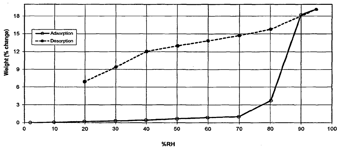
Figure 6 Sorption profile at 25°C of Modification N
