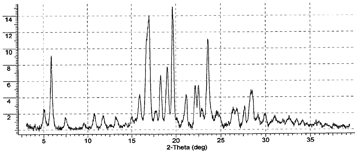
Figure 2.10: X-ray Powder Diffraction Pattern (PXRD) of Modification J
