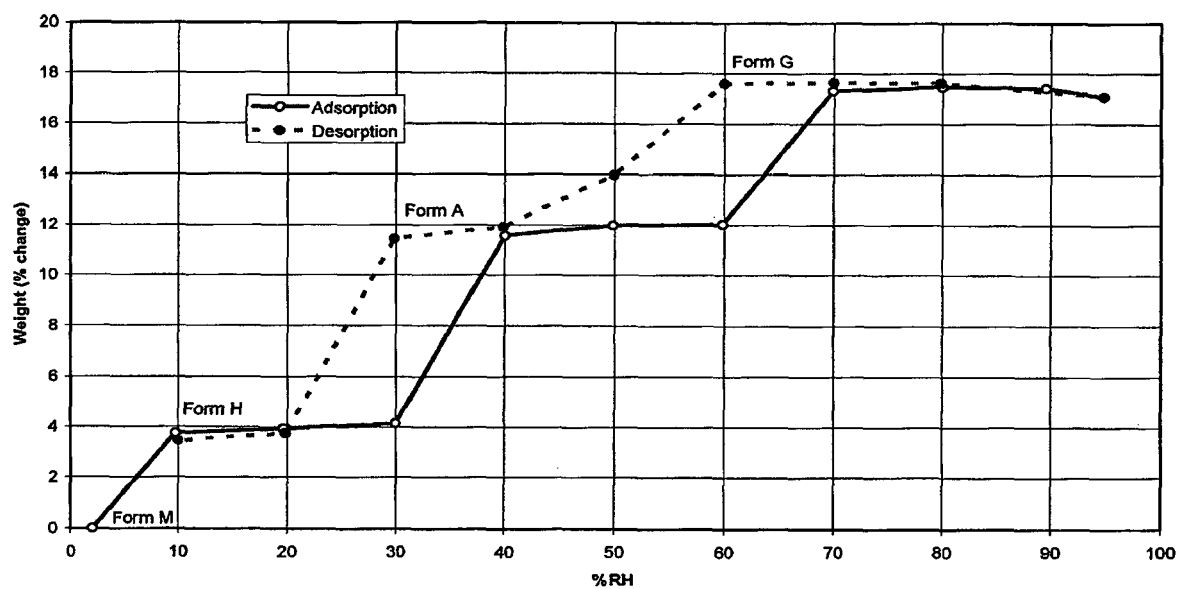
Figure 1 Sorption results of Modification A
