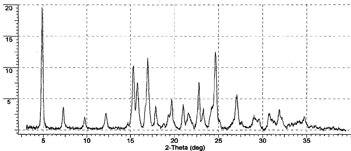
Figure 2.5 X-ray Powder Diffraction Pattern (PXRD) of Modification E
