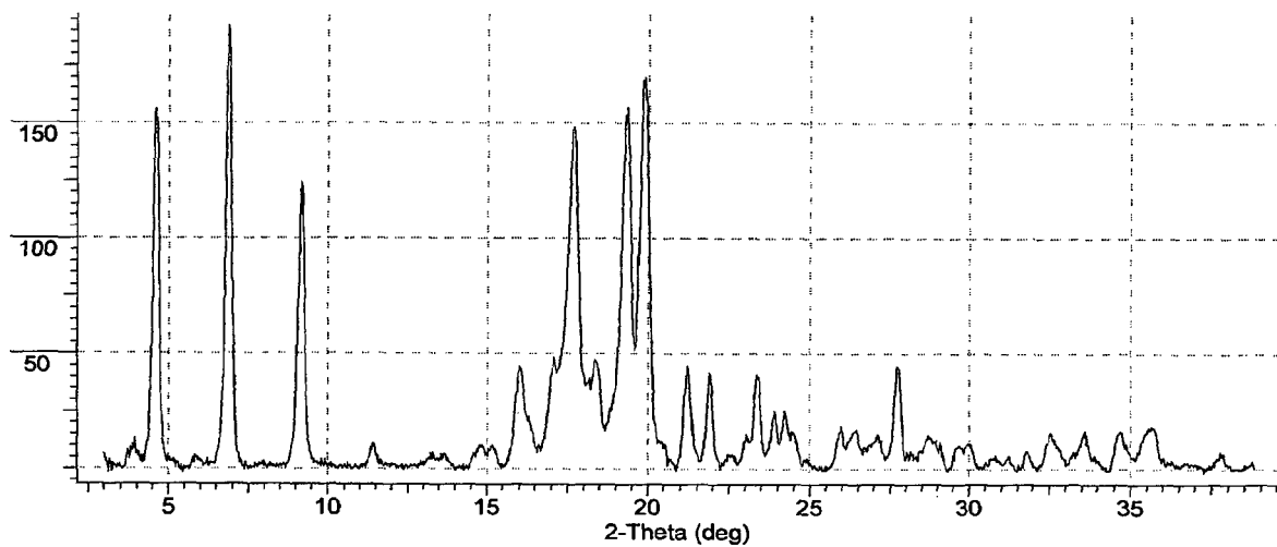
Figure 2.16 X-ray Powder Diffraction Pattern (PXRD) of Modification P
