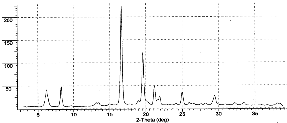
Figure 2.14 X-ray Powder Diffraction Pattern (PXRD) of Modification N
