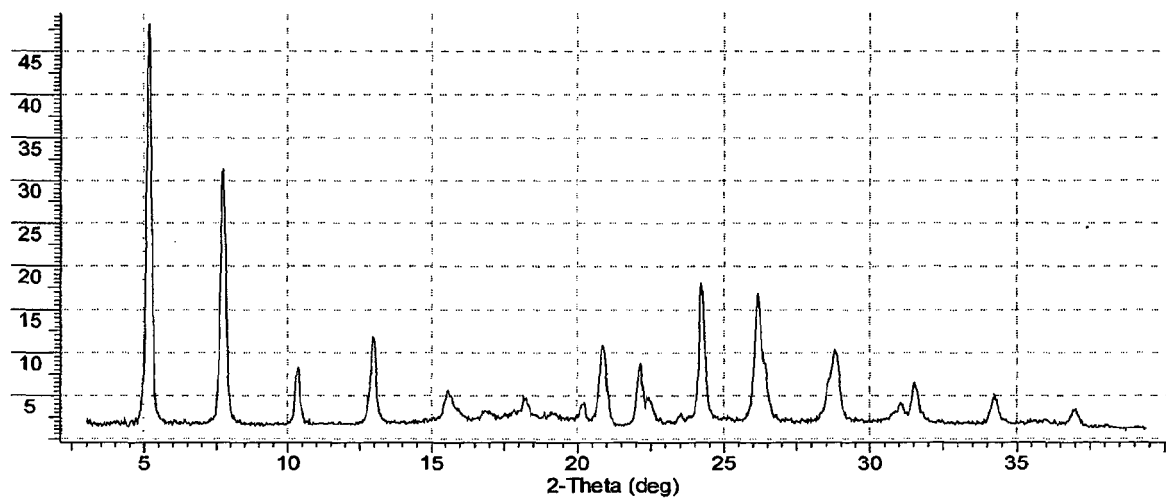
Figure 2.2: X-ray Powder Diffraction Pattern (PXRD) of Modification B
