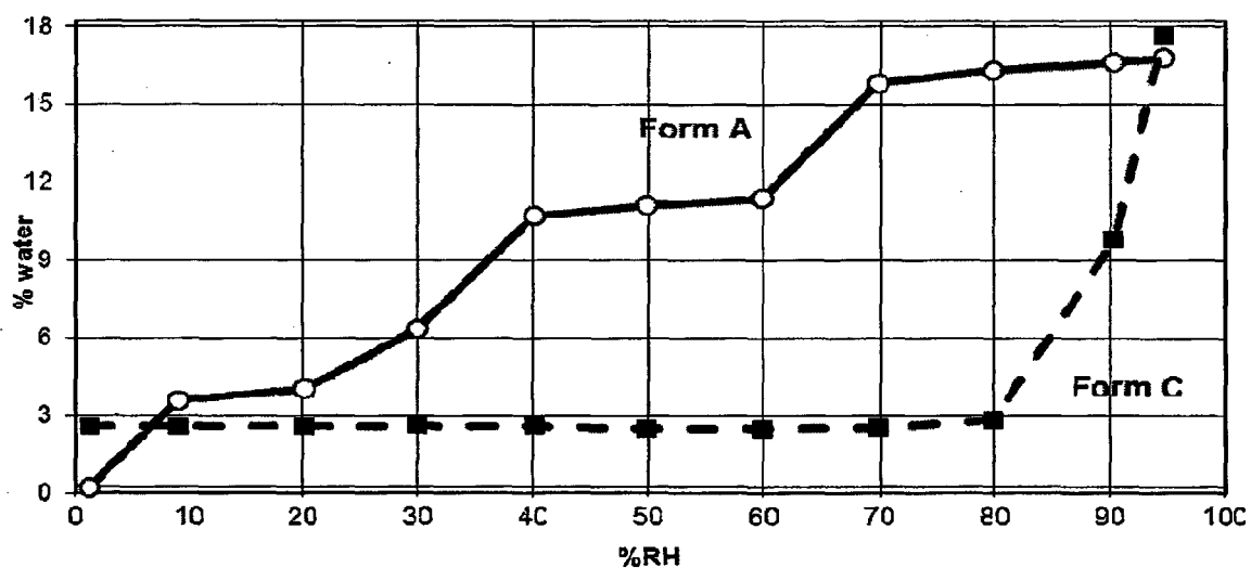
Figure 5 Sorption profile differences at 25°C between Modification A (Form A) and Modification C (Form C)
