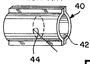
FIG. 4 PRIOR ART
