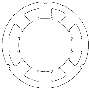
[FIG. 7(c)] 8 SLOTS (8 POLES)
