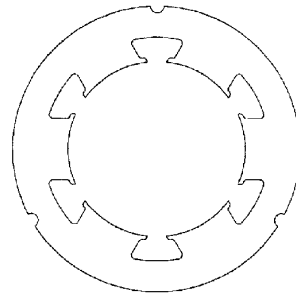
[FIG. 7(b)] 6 SLOTS (6 POLES)
