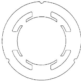
[FIG. 7(a)] 4 SLOTS (4 POLES)
