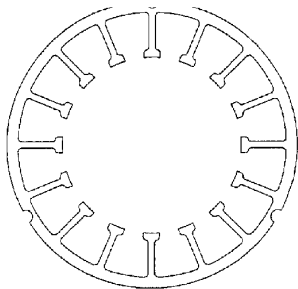
[FIG. 7(g)] 16 SLOTS (16 POLES)
