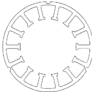
[FIG. 7(f)] 14 SLOTS (14 POLES)
