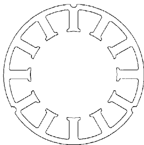
[FIG. 7(e)] 12 SLOTS (12 POLES)
