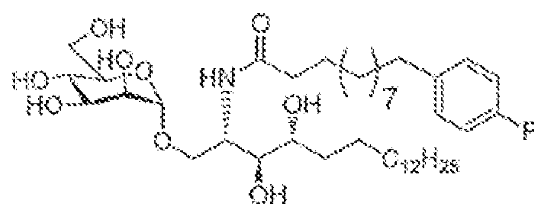
7DW8-5-Man
