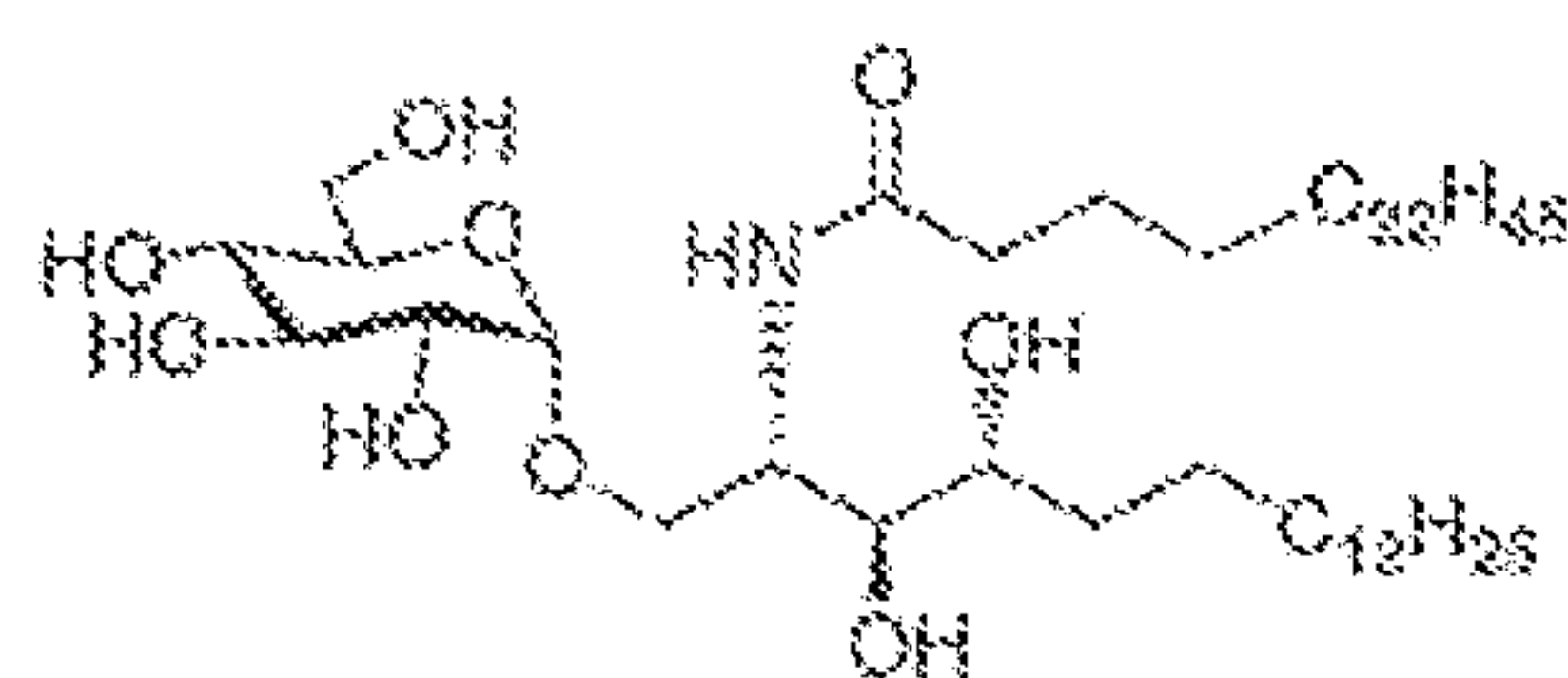
C1-Glc (Compound 24)
