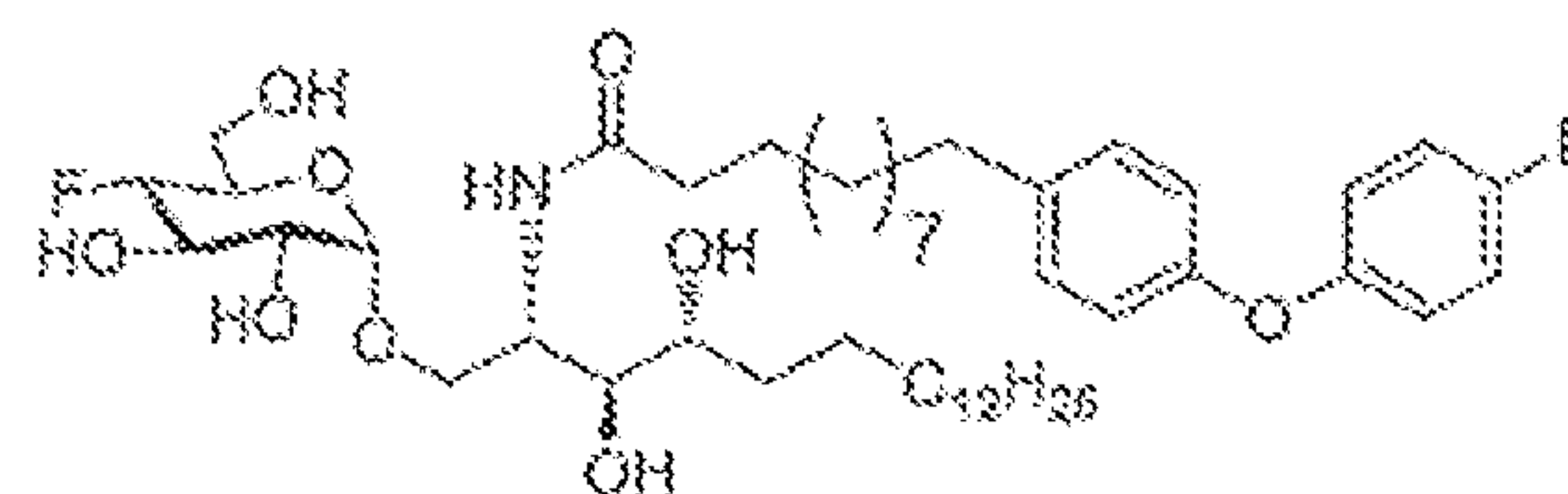
Compound 43
