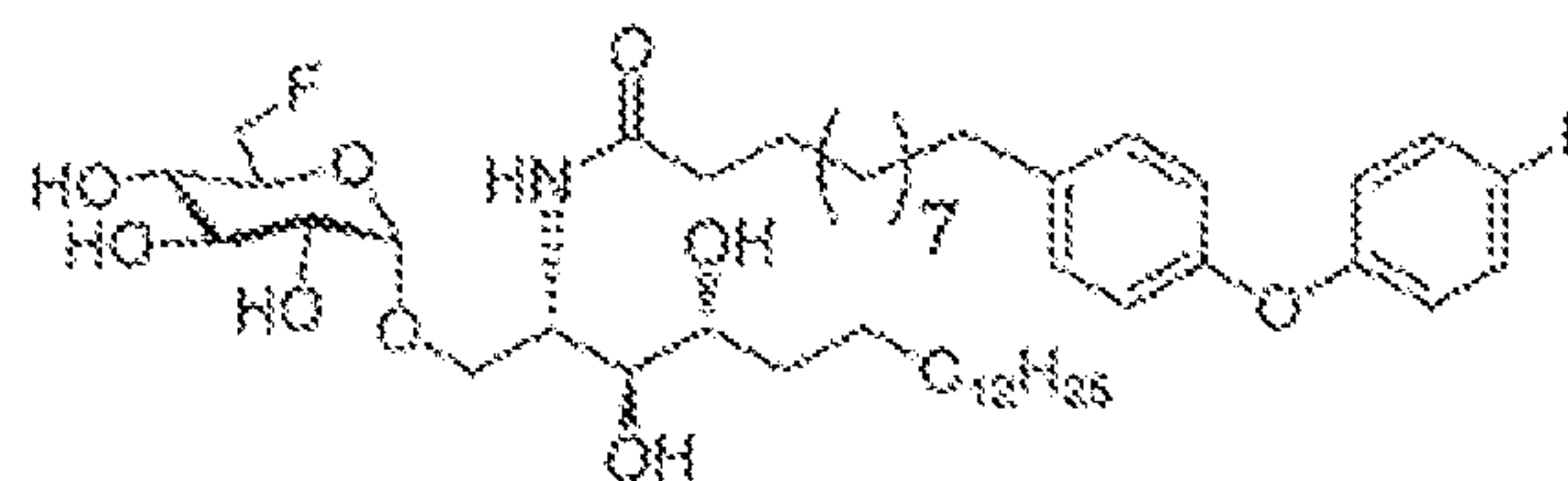
Compound 53
