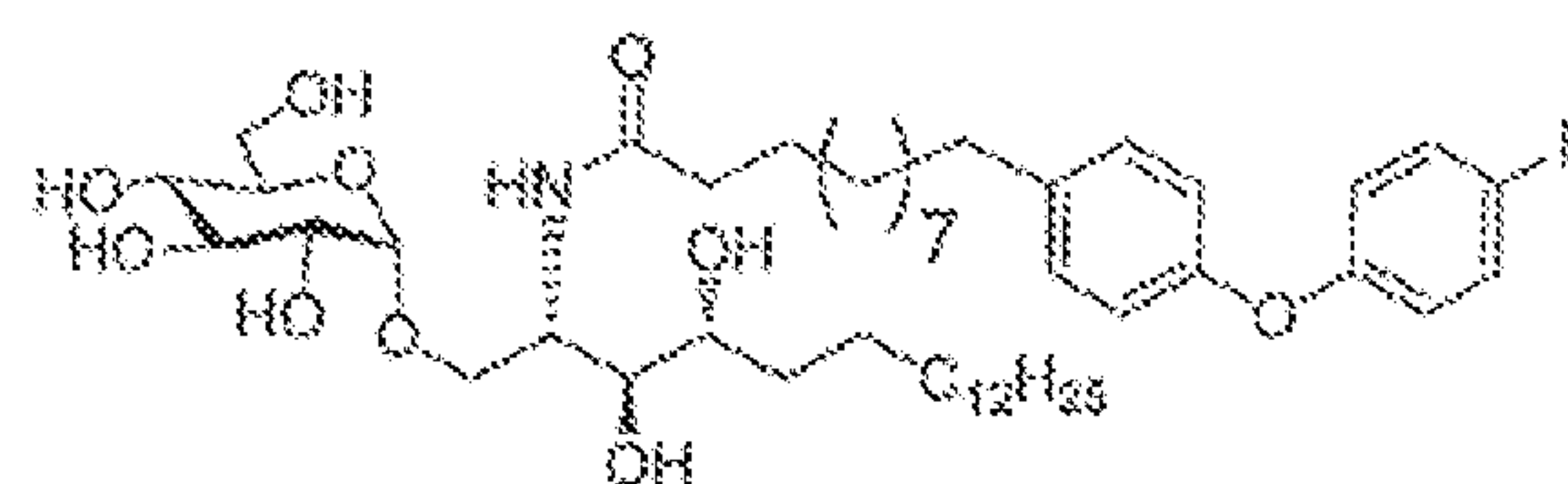
C34-Glc (Compound 26)
