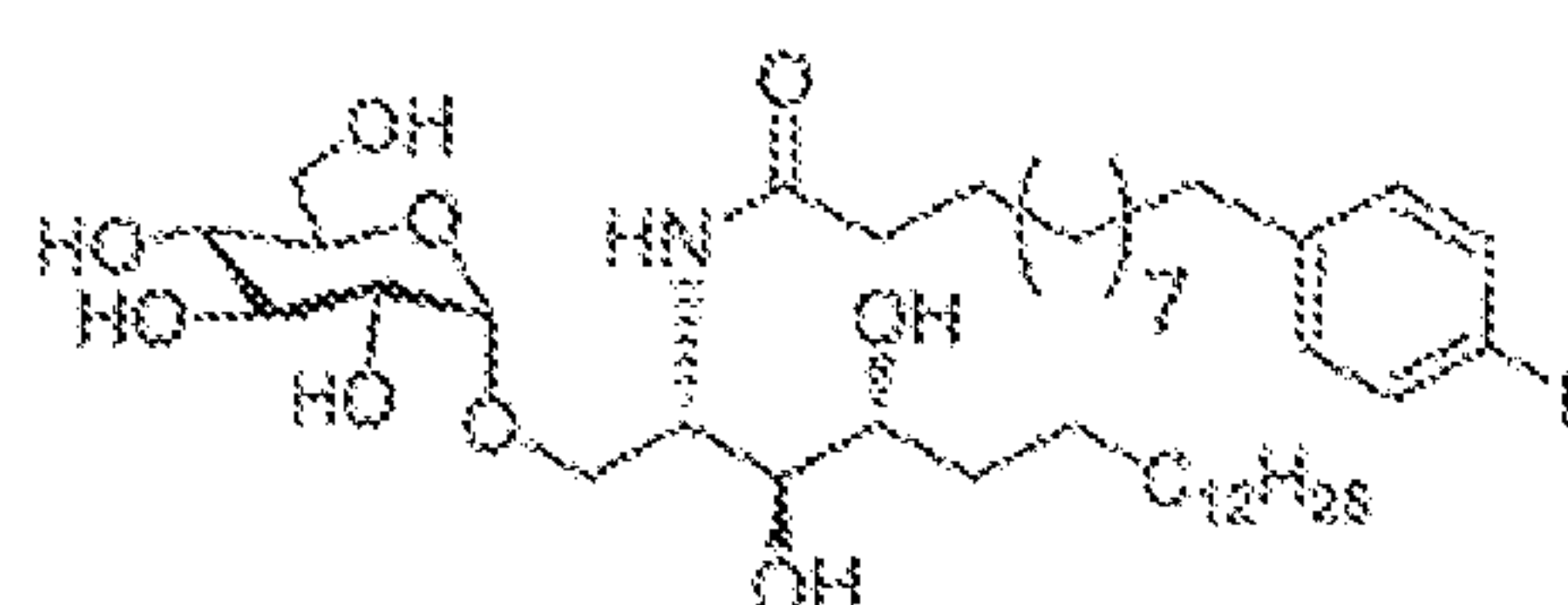
7DW8-5-Glc (Compound 25)
