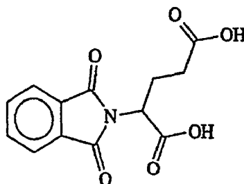
phthaloyl glutamic acid (PG Acid)
