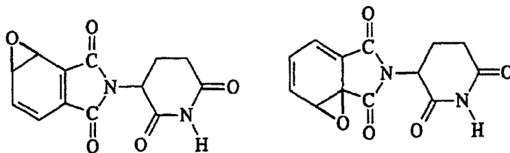
Epoxides of thalidomide
