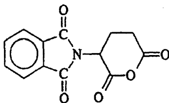
phthaloyl glutamic anhydride (PGA)
