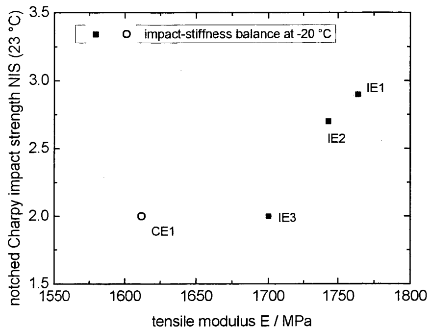
- - Figure 2: Impact stiffness balance at -20 °C
