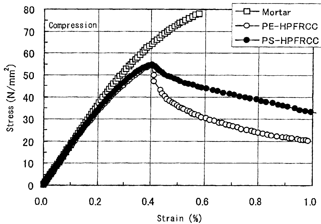
Stress—strain diagram in compression test
