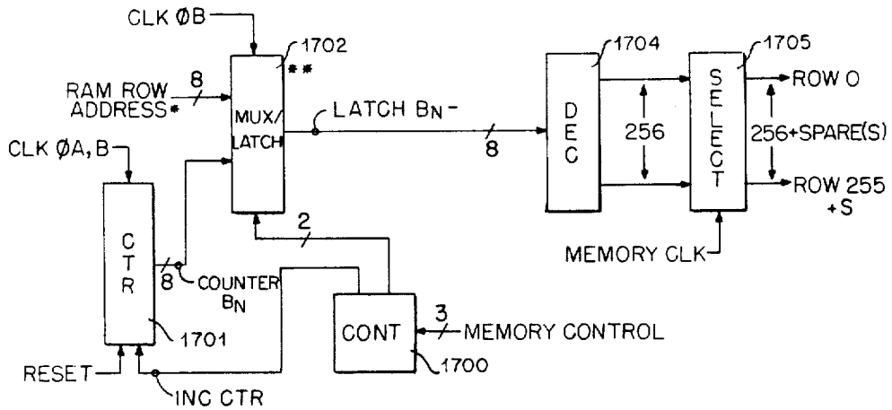
FIG. 14A. BLOCK DIAGRAM
