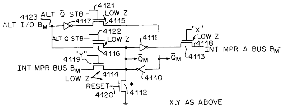
MPR FIG. 20 B. ALTERNATE INPUTS
