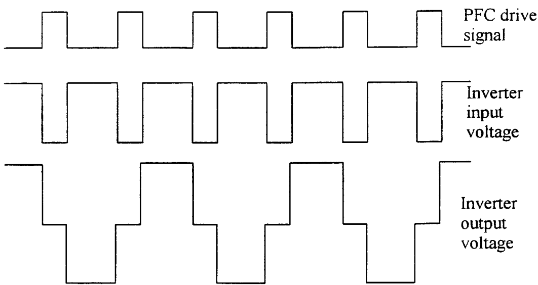
Inverter input and output waveforms
