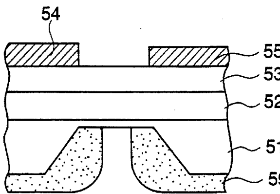
Fig.11 (c) Prior Art
