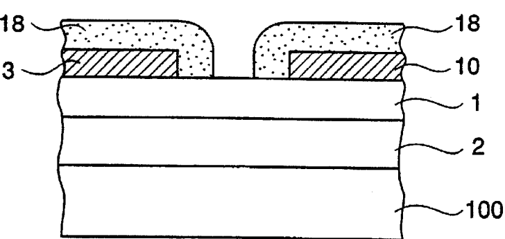
Fig.9(c) Prior Art
