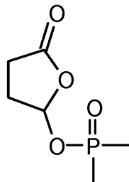
2-oxotetrahydrofuran-5-yl E-2
