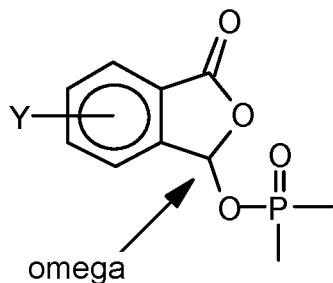
3-phthalidyl E-1
