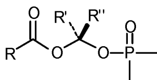
Formula A
