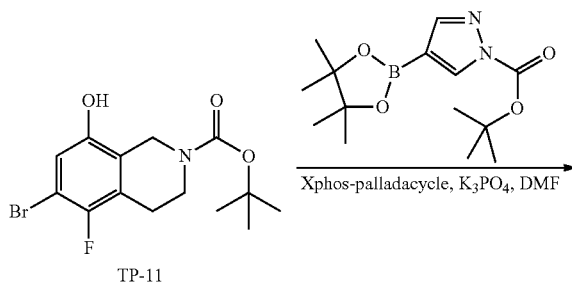
Scheme MMM
