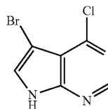
5-bromo-4-chloro-7H-pyrrolo[2,3-d]pyrimidine
