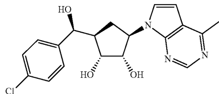
Example 11: 4-chloro- phenyl magnesium bromide
