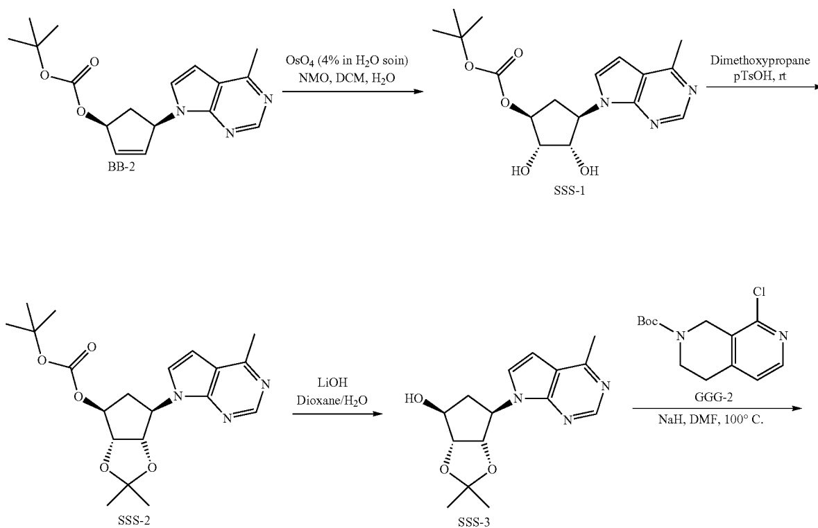
Scheme SSS
