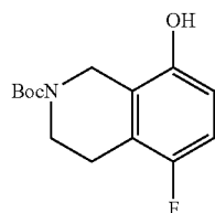
Example 100 TP-2
