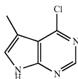
Example 123 TP-5
