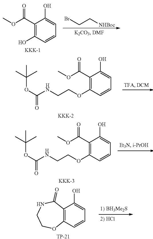
Scheme KKK
