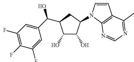
Example 13: 3,4,5- trifluoro- phenyl magnesium bromide
