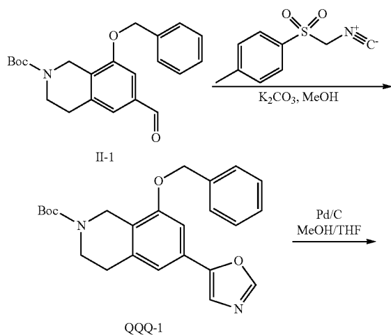
Scheme QQQ
