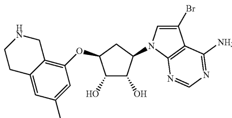
474 M + 1
