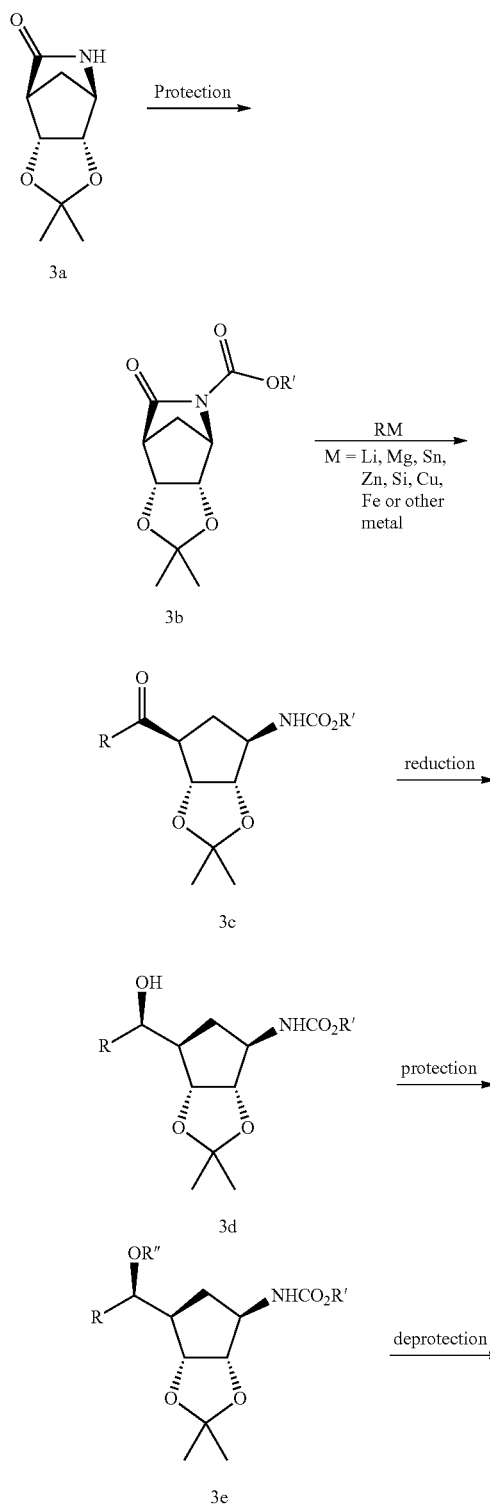
Scheme 3:
