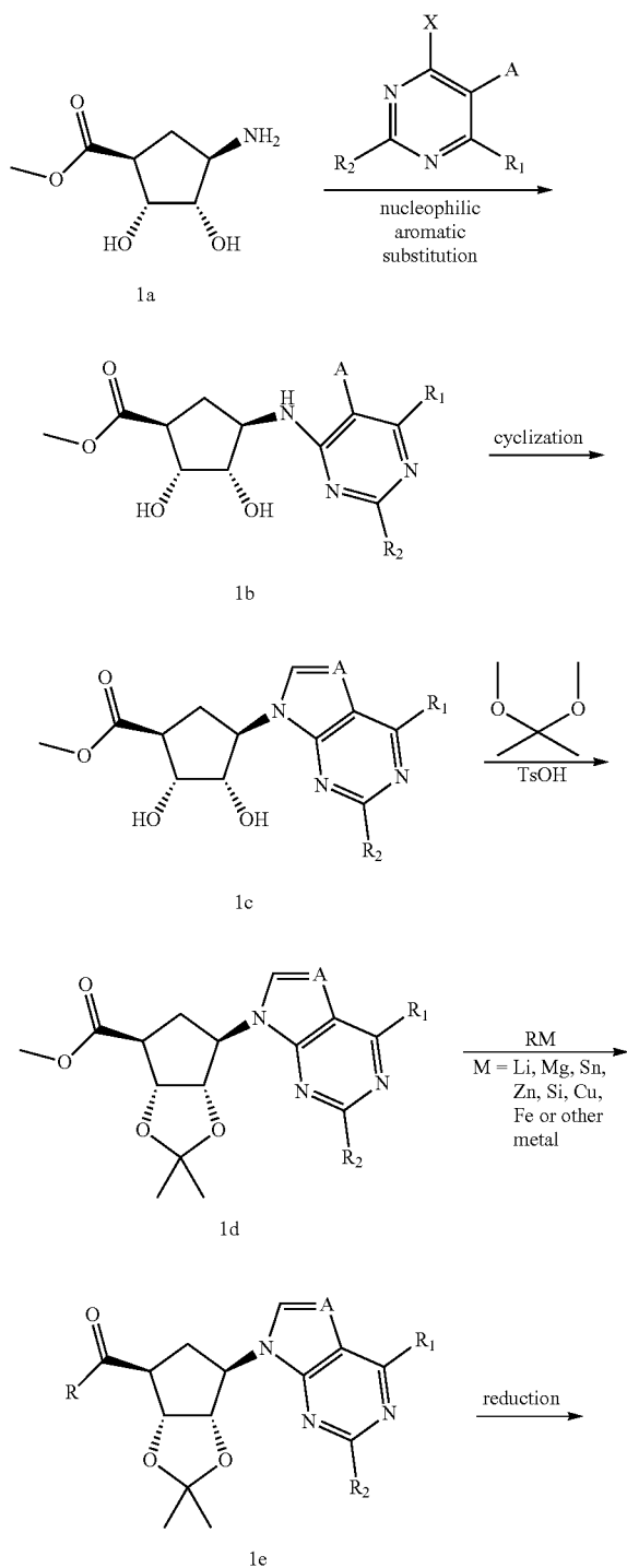
Scheme 1:
