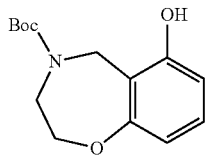
Example 164 TP-22
