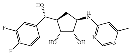
Example 34 4-chloro-6-methylpyrimidine
