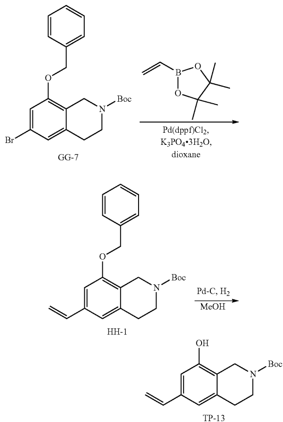
Scheme HH
