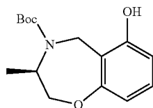
TP-45
