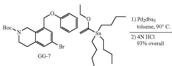
Scheme RRR
