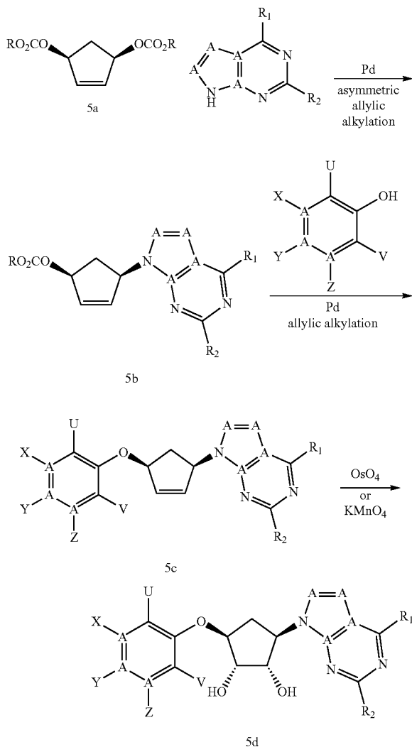
Scheme 5:
