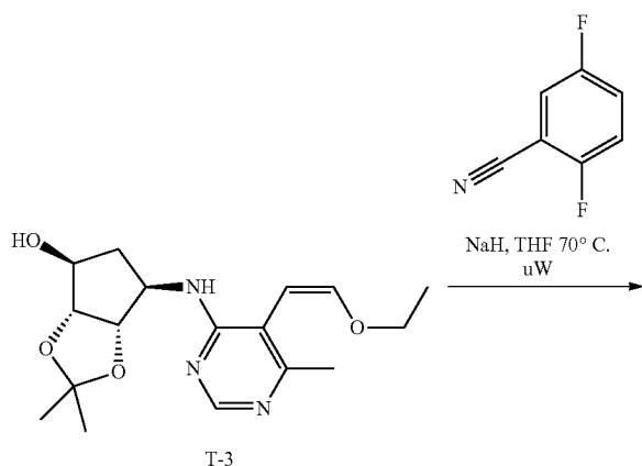
Scheme X
