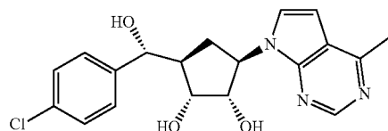
Example 12: 4-chloro- phenyl magnesium bromide
