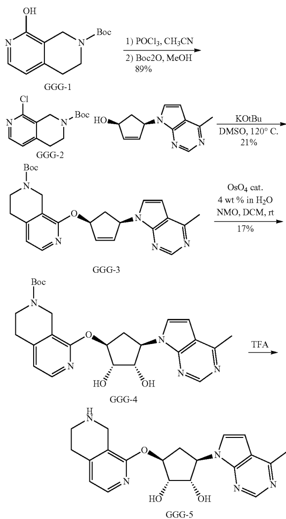
Scheme GGG
