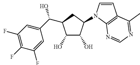
Example 14: 3,4,5- trifluoro- phenyl magnesium bromide
