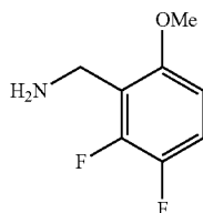
Example 145 (2,3-difluoro-6-methoxyphenyl)methanamine
