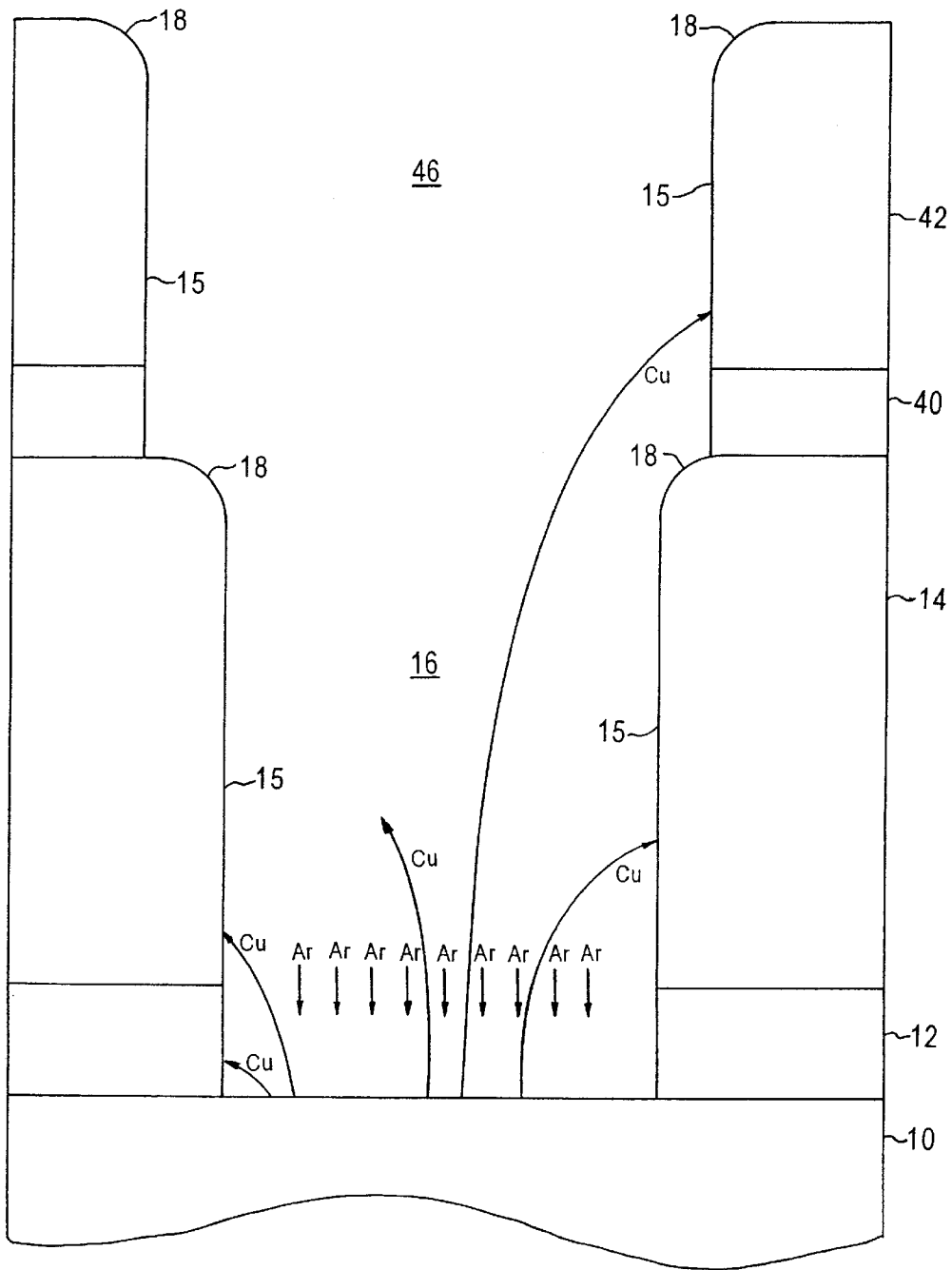
FIG. 3 (PRIOR ART)
