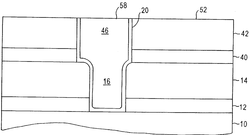
FIG. 2L (PRIOR ART)
