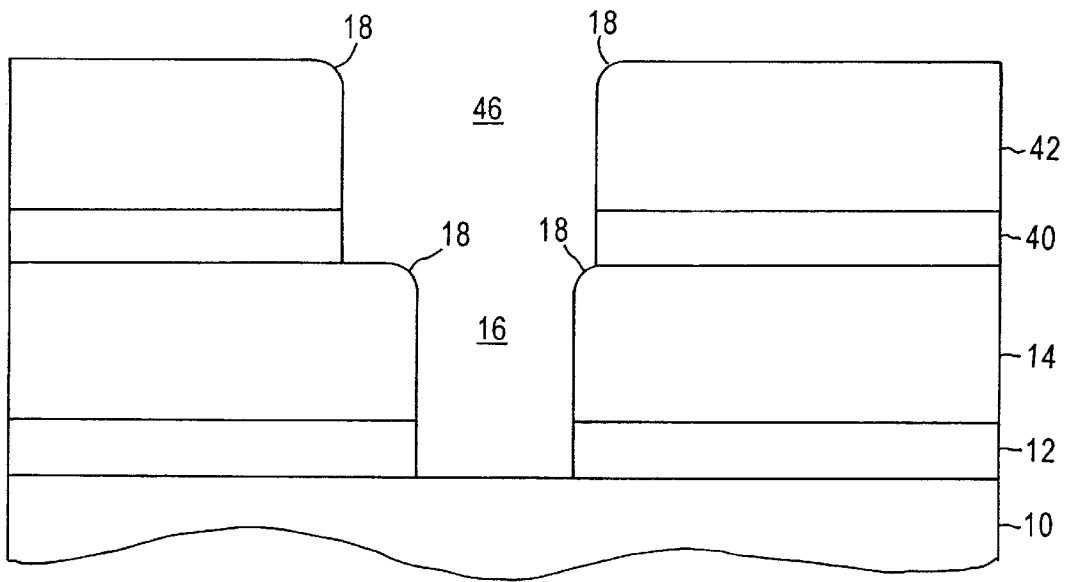
FIG. 2I (PRIOR ART)
