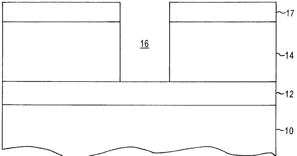
FIG. 1C (PRIOR ART)
