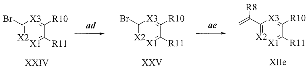
Scheme XVIII
