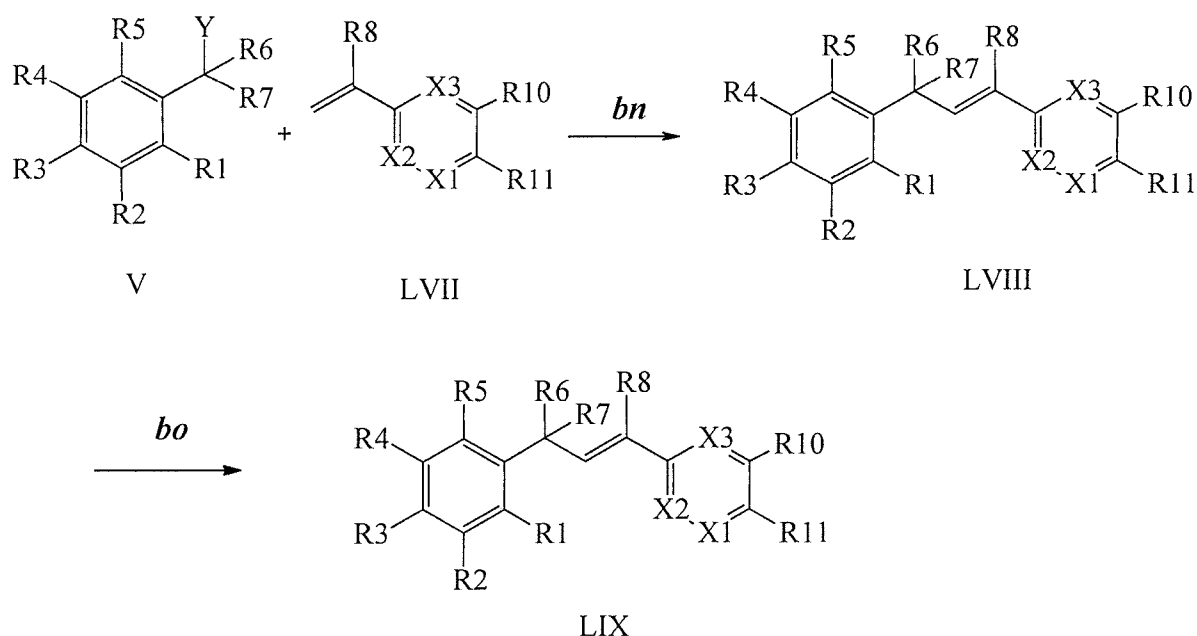
Scheme XL
