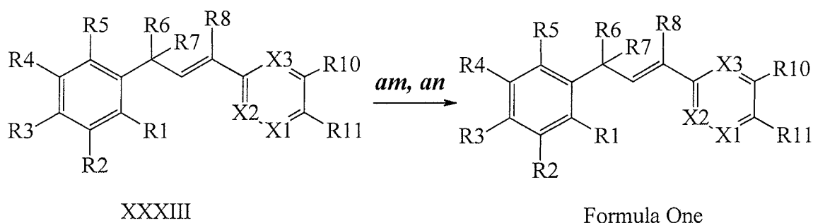
Scheme XXX
