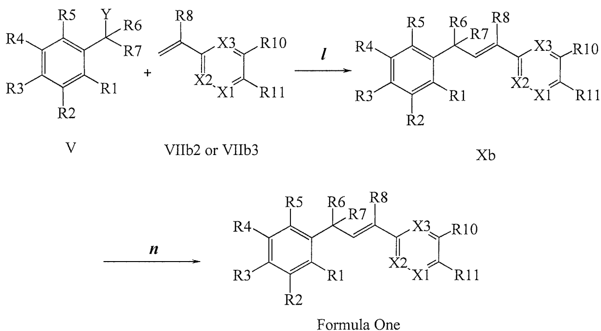
Scheme VIII
