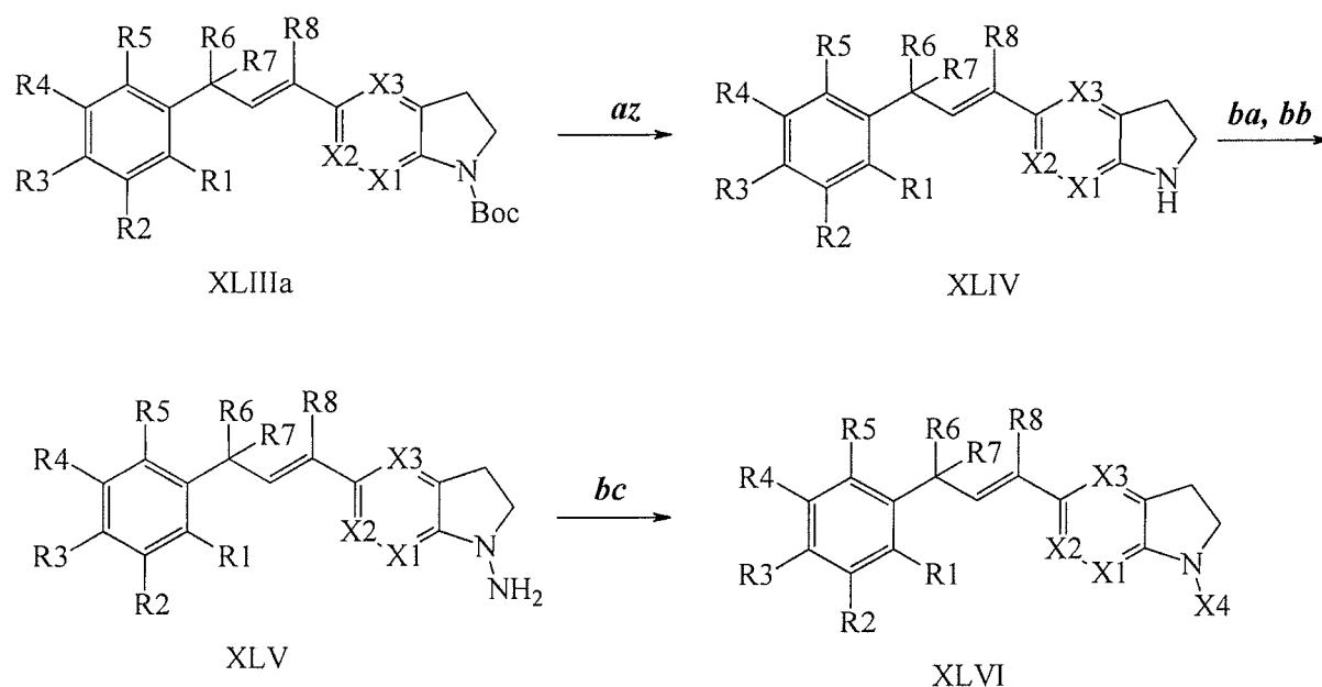
Scheme XXXVI
