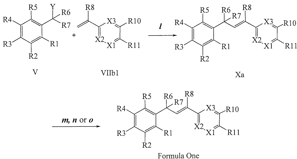
Scheme VII
