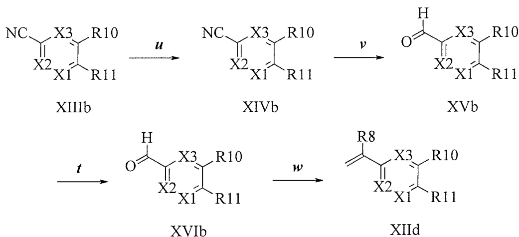
Scheme XVII
