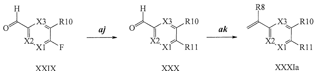
Scheme XXVII
