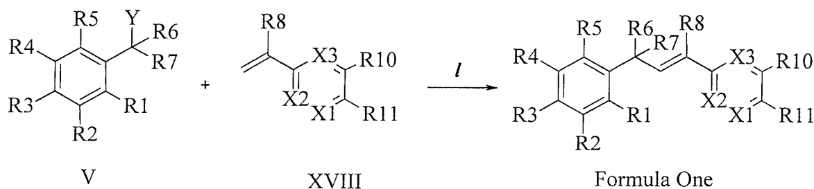
Scheme XXVI
