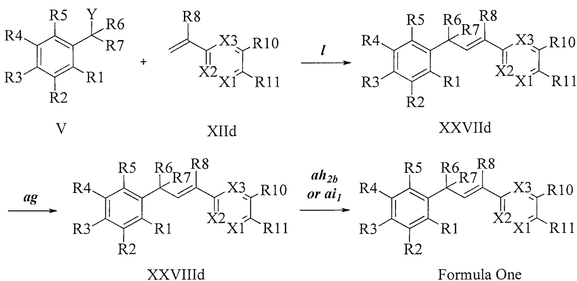
Scheme XXIII
