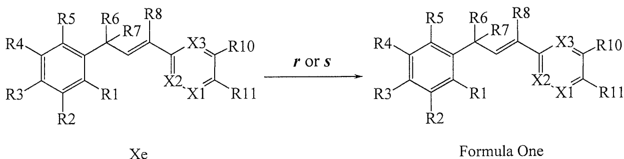
Scheme XII
