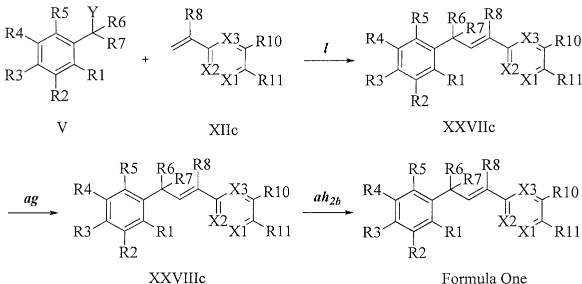
Scheme XXII
