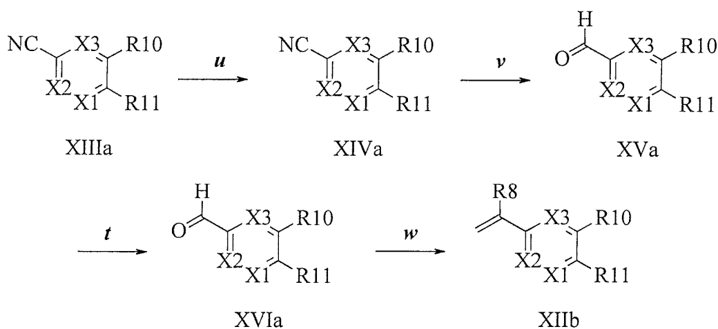
Scheme XIV
