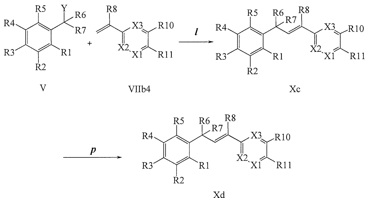
Scheme X
