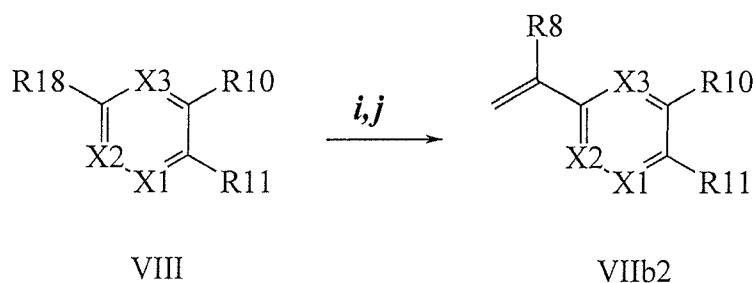
Scheme IV
