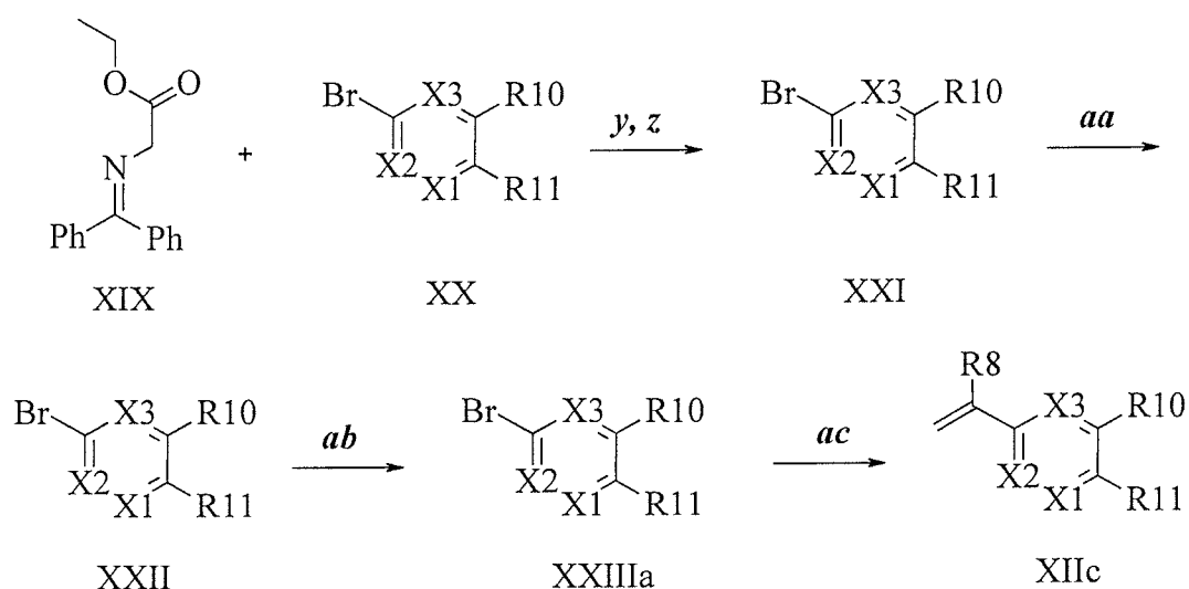
Scheme XVI
