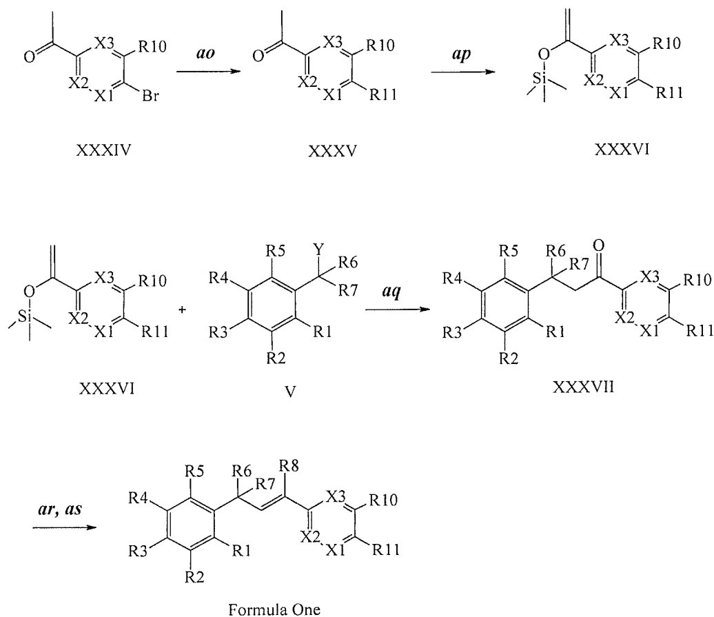
Scheme XXXI
