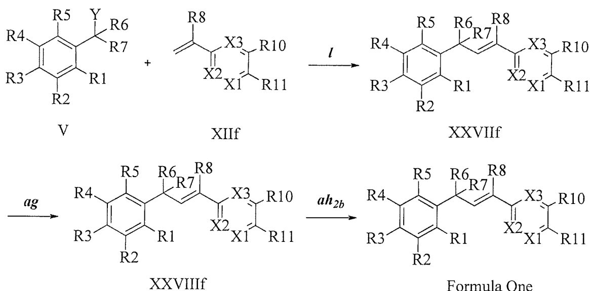
Scheme XXV
