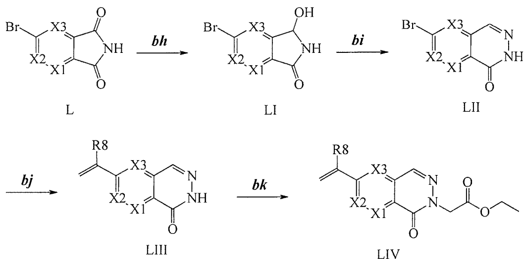
Scheme XXXVIII
