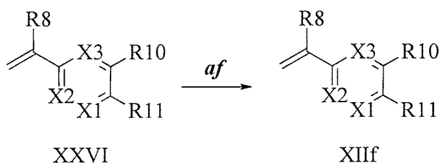
Scheme XIX
