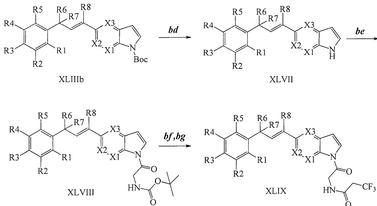
Scheme XXXVII
