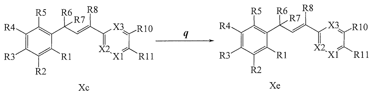
Scheme XI
