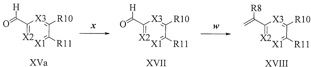
Scheme XV
