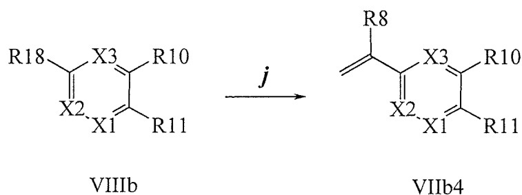
Scheme IX
