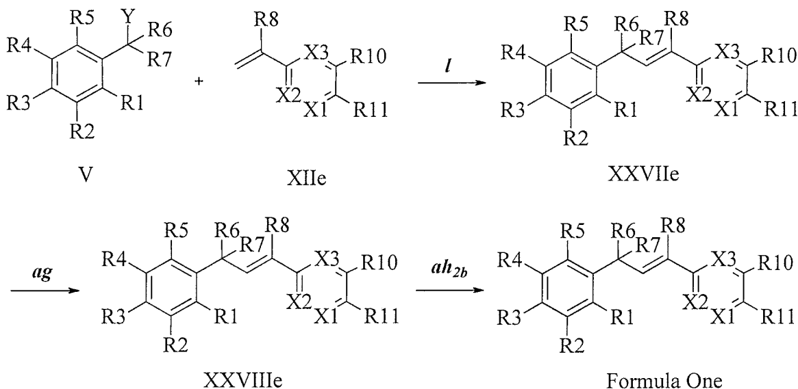
Scheme XXIV
