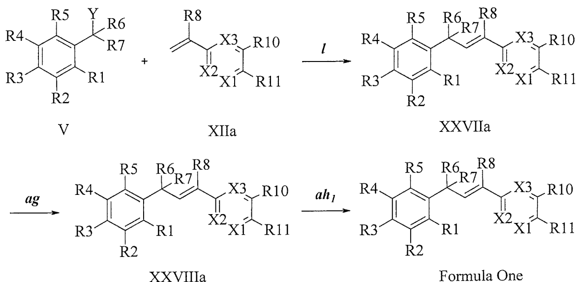
Scheme XX
