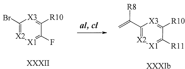
Scheme XXVIII
