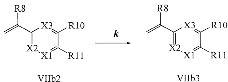
Scheme V
