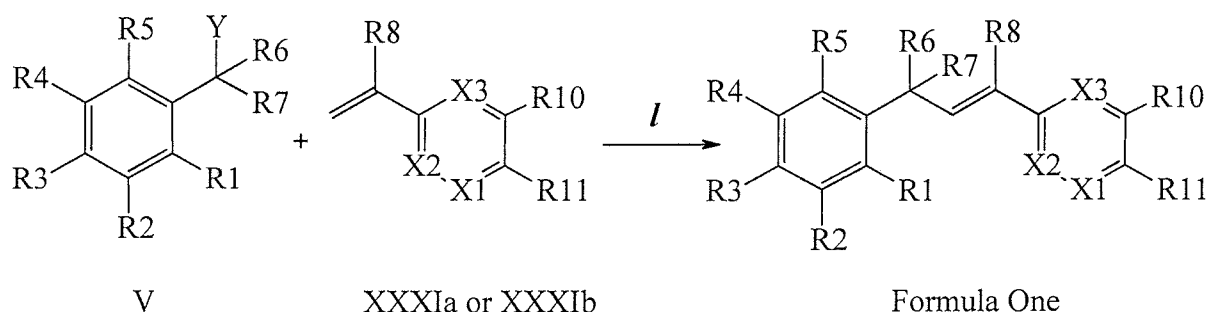
Scheme XXIX
