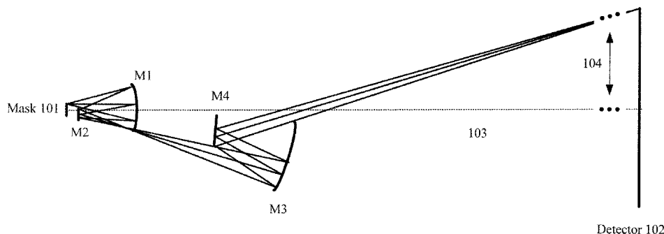
Inspection system 100
