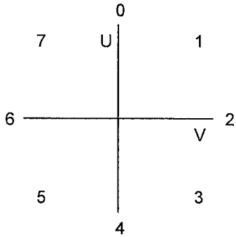
Divergent Spherical: Positive Axes
