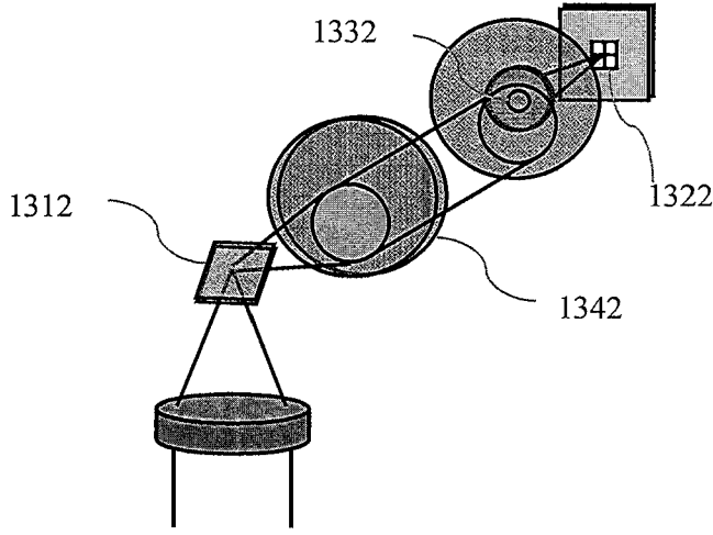
Wavefront Source being measured
