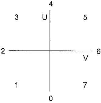
Convergent Spherical: Negative Axes
