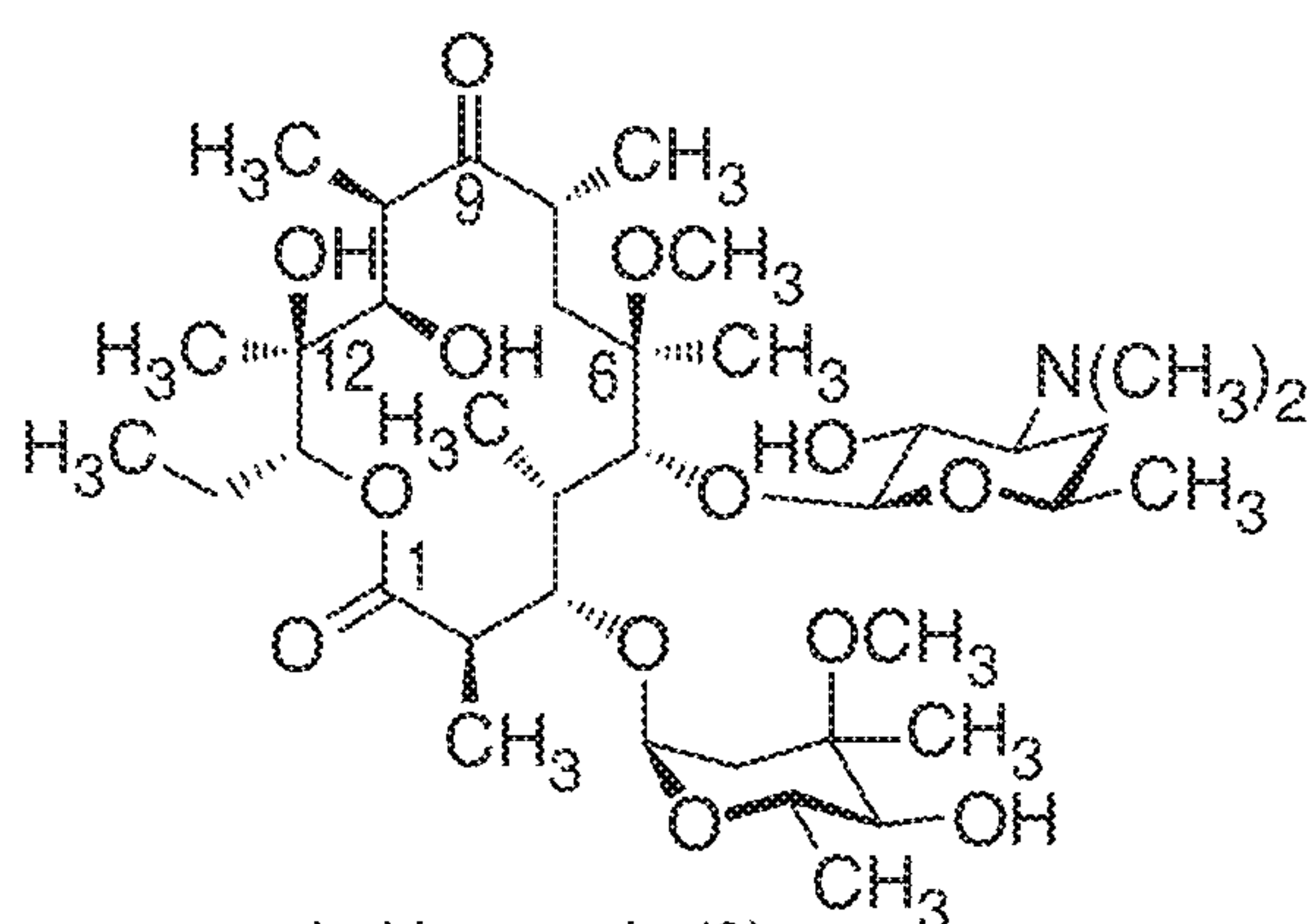
clarithromycin (2)
