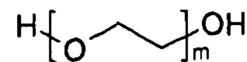
polyethylene glycol
