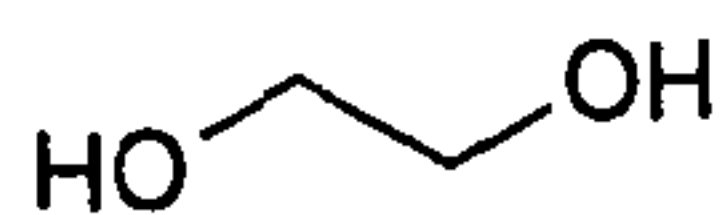
ethylene glycol
