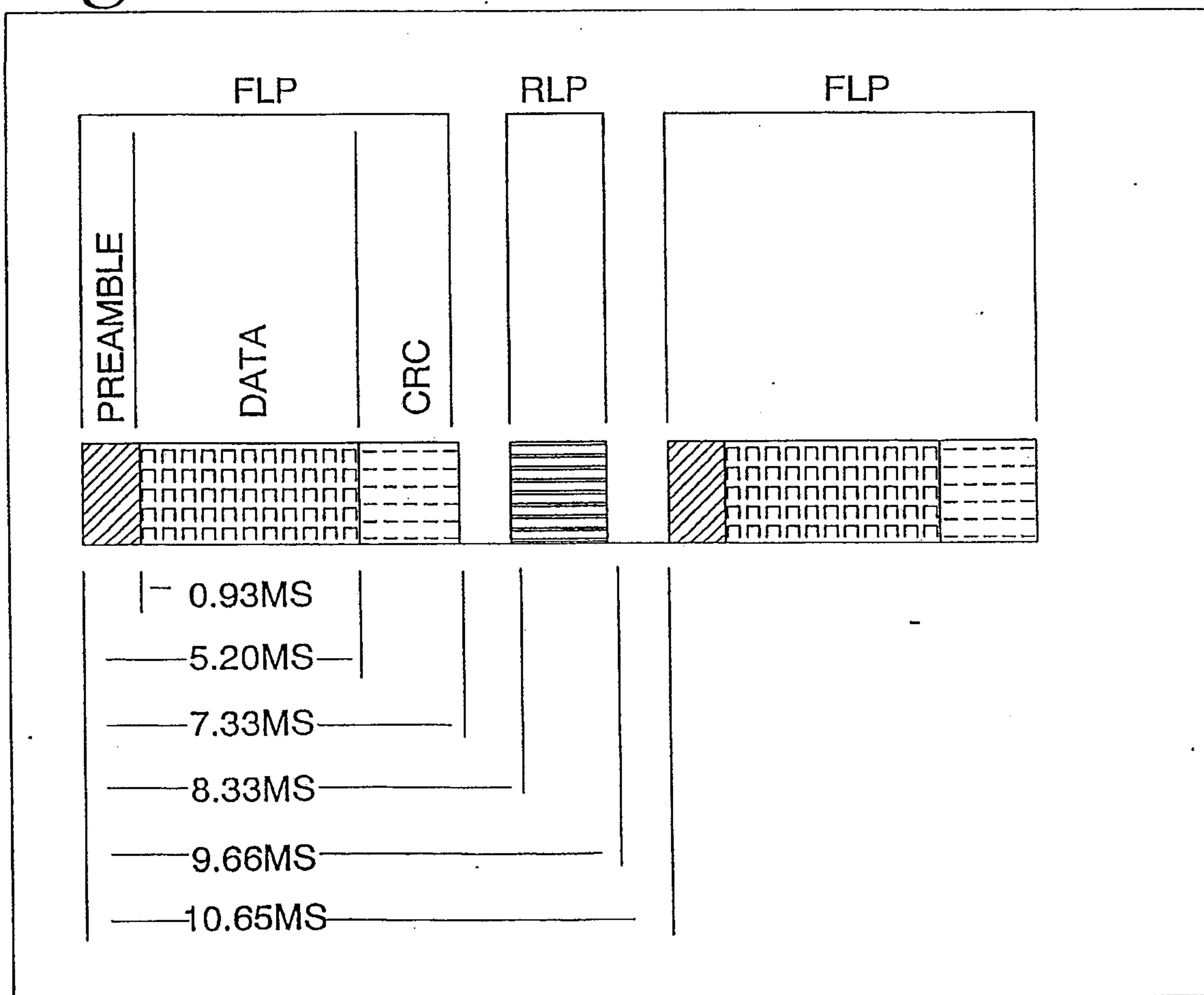
TIMING DIAGRAM WITH PREAMBLE &amp; CRC
