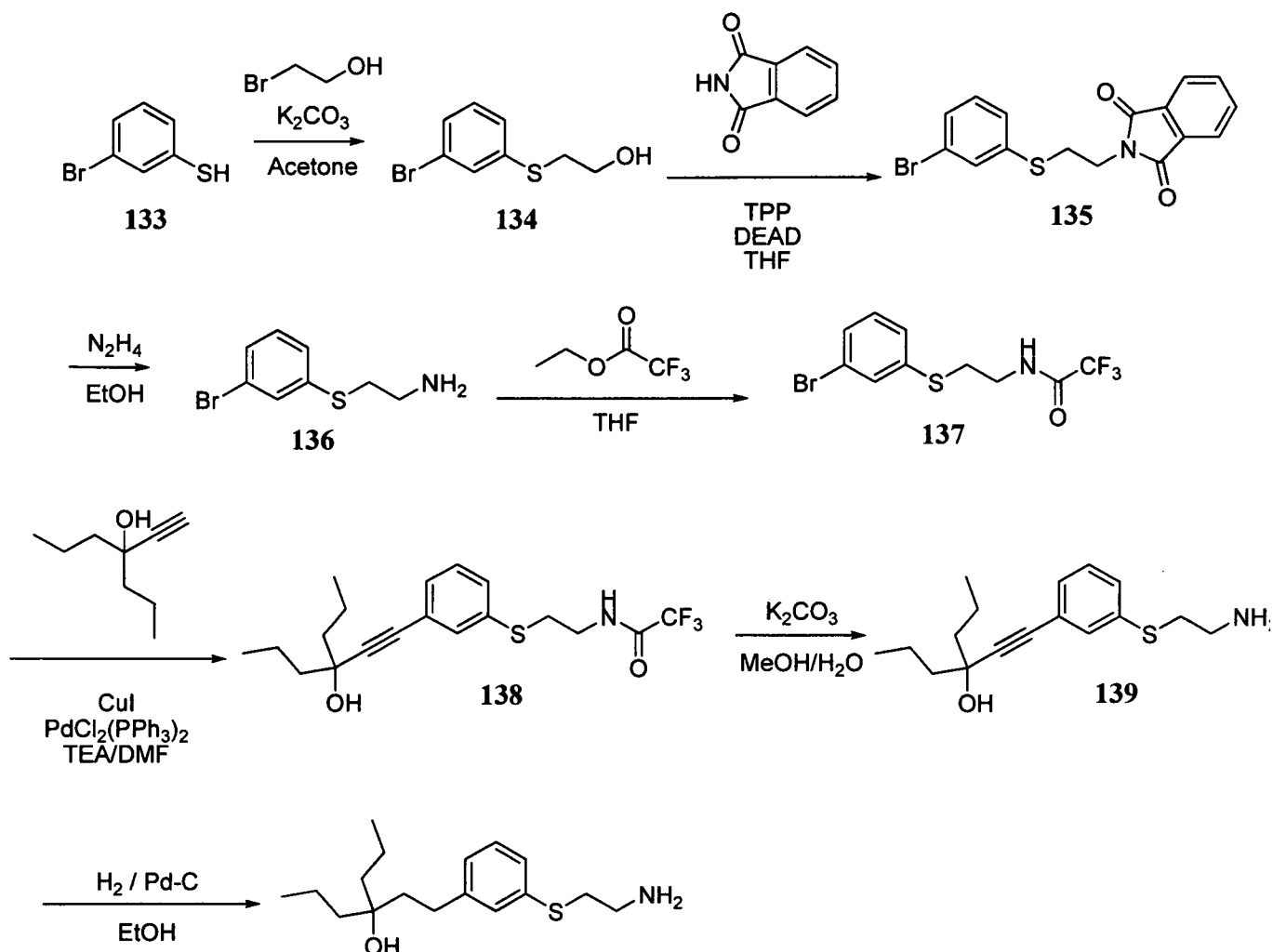
SCHEME 26
