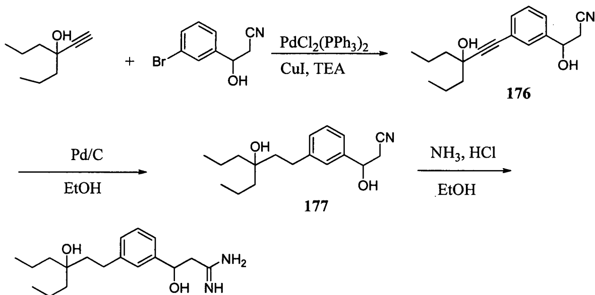
SCHEME 36
