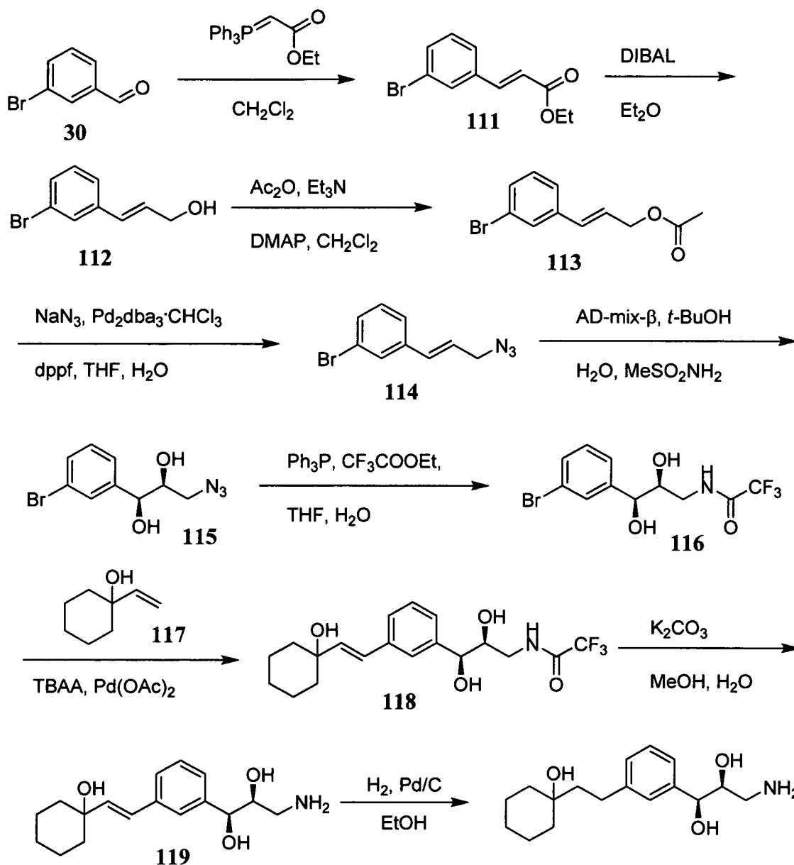
SCHEME 23
