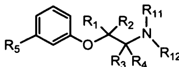
Formula (Ib)
