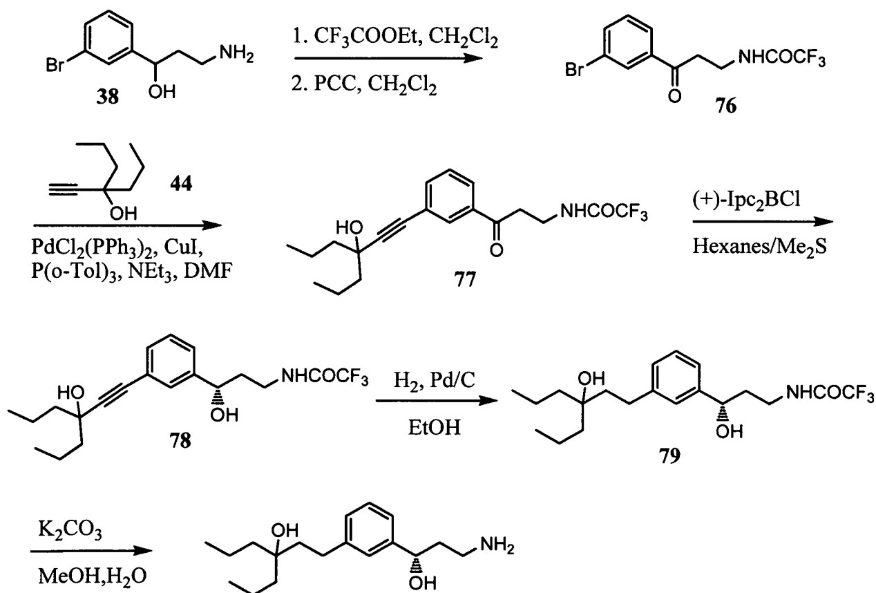
SCHEME 16
