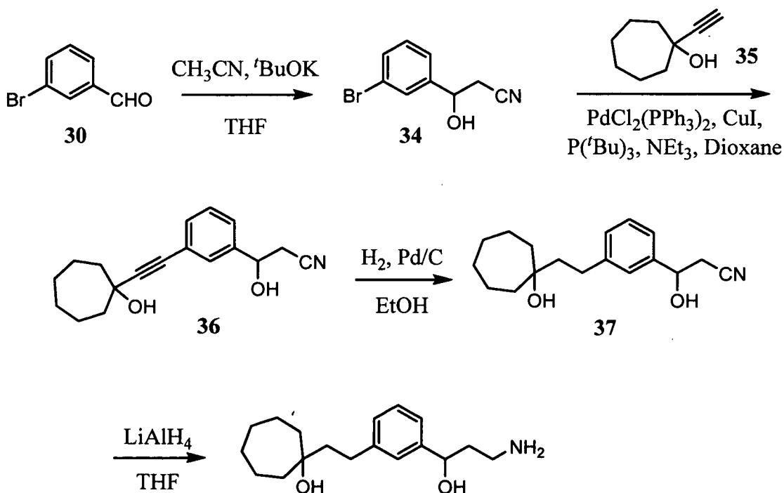
SCHEME 7
