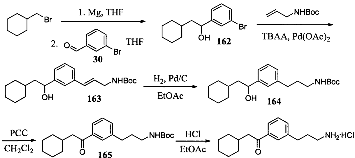
SCHEME 32
