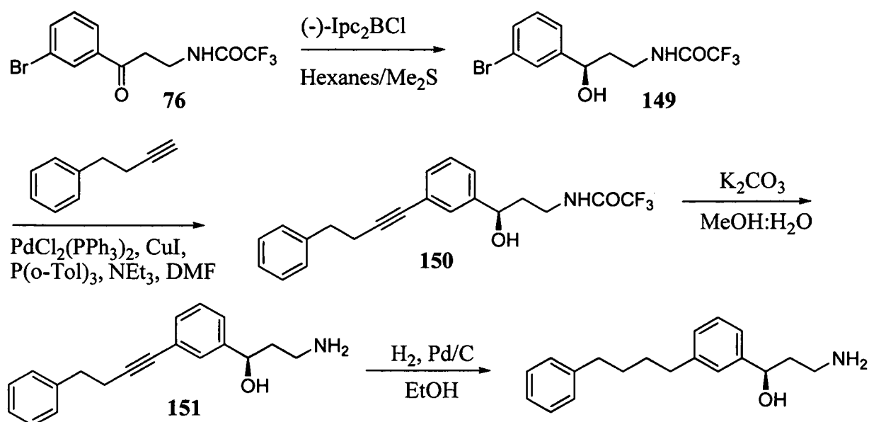
SCHEME 29
