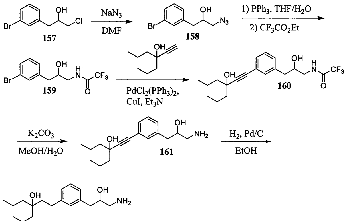
SCHEME 31
