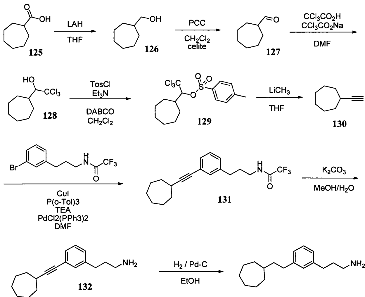
SCHEME 25
