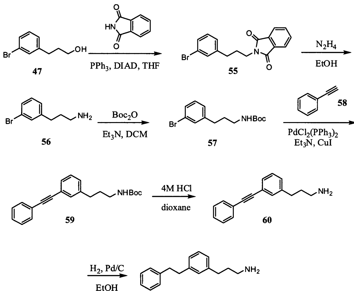
SCHEME 11
