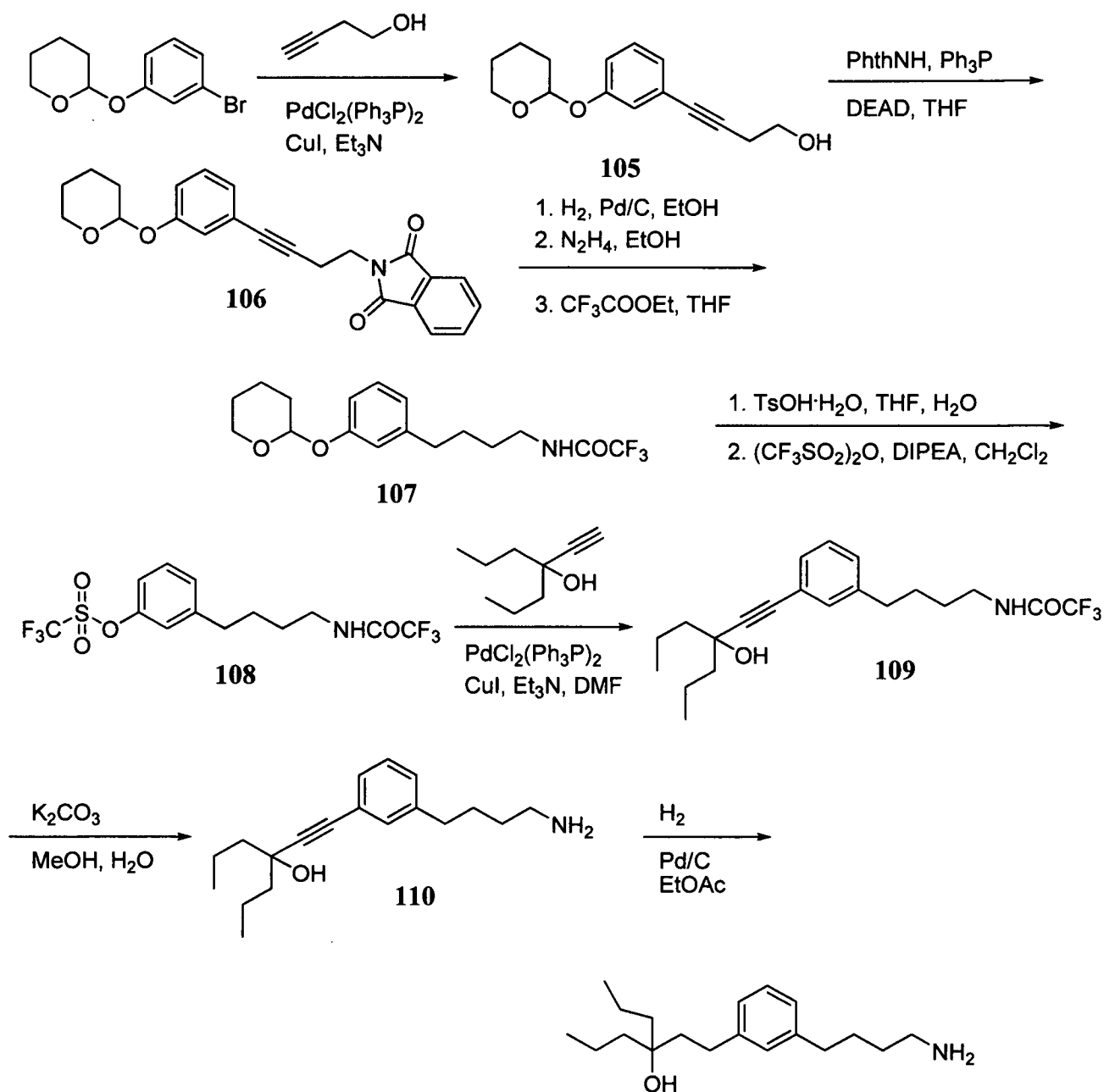
SCHEME 22
