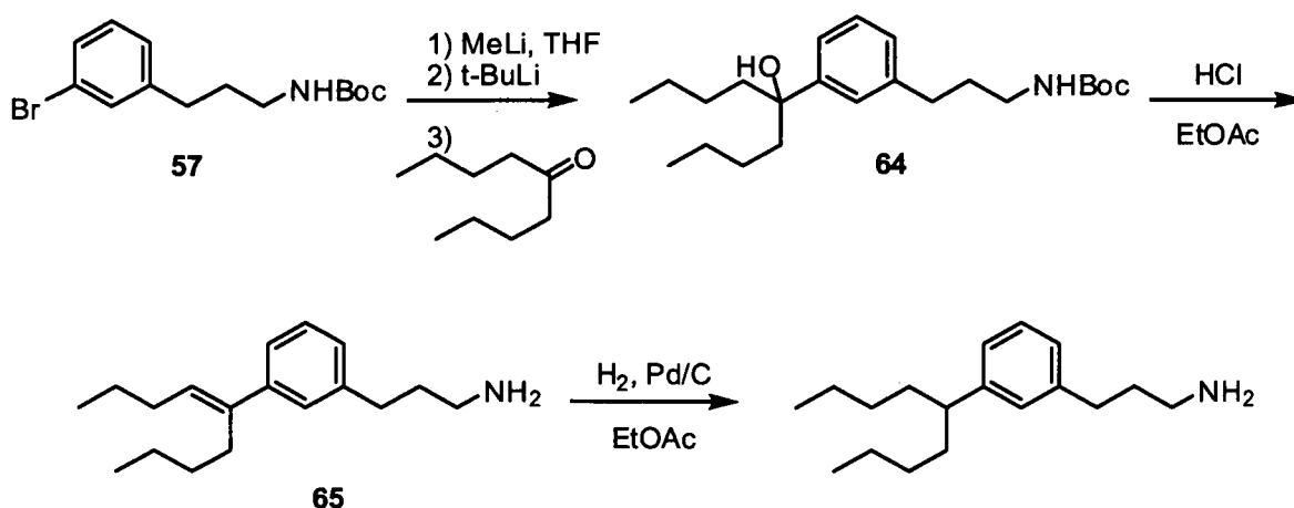
SCHEME 13
