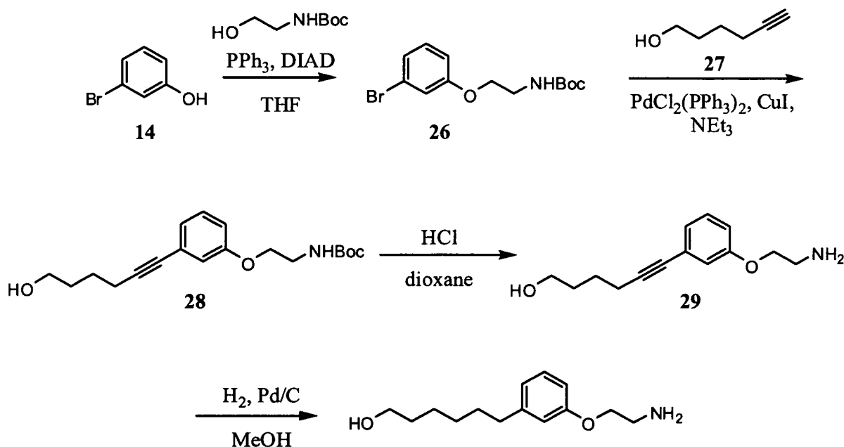
SCHEME 5
