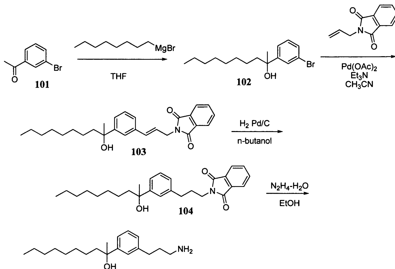
SCHEME 21
