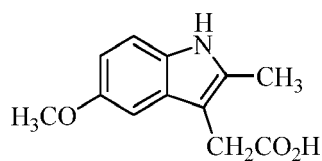
Compound 11
