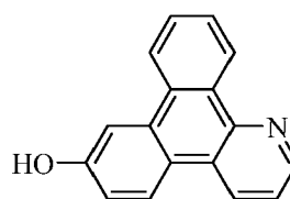
Compound 10
