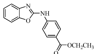
Compound 16
