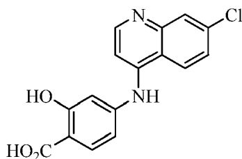
Compound 15
