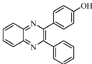
Compound 3
