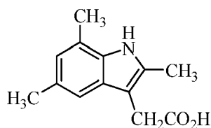
Compound 14
