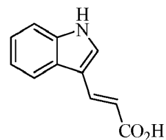
Compound 13
