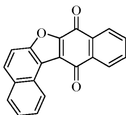
Compound 9
