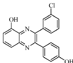
Compound 7
