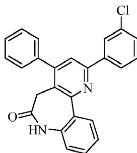
Compound 12
