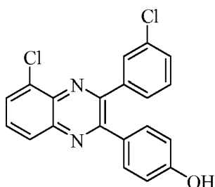
Compound 5
