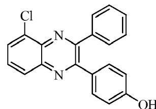
Compound 4
