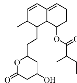
Compound 19
