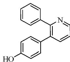
Compound 1 .
