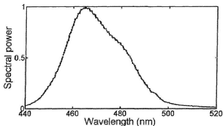
Figure 3.5. Measured LED illumination output spectral profile.
