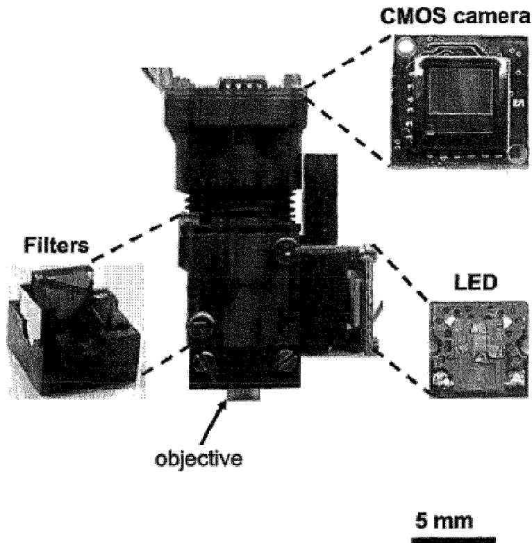
Figure 4.1. A typical fabricated miniature fluorescence microscope with main components labeled. The scale bar applies to main photograph and all insets.
