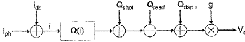
Figure 3.14. CMOS image sensor signal and additive noise model.
