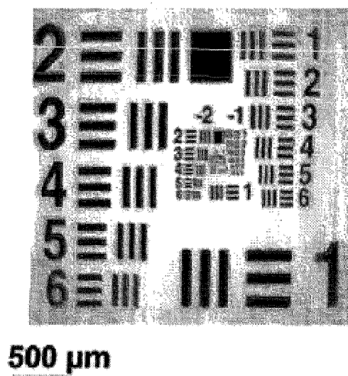
Figure 3.11. Optical image irradiance of the USAF 1951 resolution target. Optical image dimensions are approximately 2.5 mm \times 2.5 mm, corresponding to an optical magnification of 5x. The imaging optics model used is based on the design of the imaging pathway presented in Section 3.1.1.
