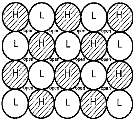
FIG. 64F: CIRCULAR VARIATION #1 (ORTHOGONAL GRID GEOMETRY)
