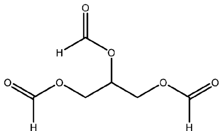
Glycerol Formates
