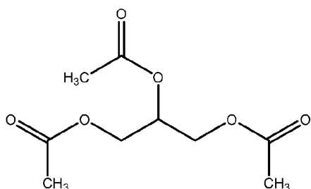
Triacetin
