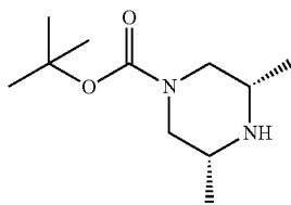
tert-Butyl (3R,5S)-3,5-dimethylpiperazine-1-carboxylate (30)
