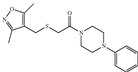
2-(((3,5-Dimethylisoxazol-4-yl)methyl)thio)-1-(4-phenylpiperazin-1-yl)ethanone (5a)
