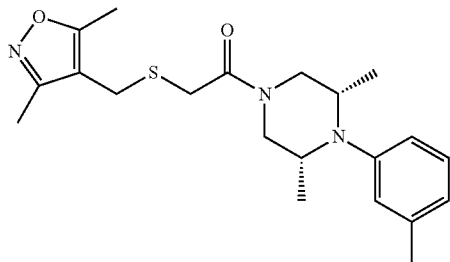
1-(3,5-Dimethyl-4-(m-tolyl)piperazin-1-yl)-2-(((3,5-dimethylisoxazol-4-yl)methylthio)ethan-1-one (5m)
