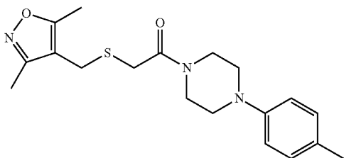
2-(((3,5-Dimethylisoxazol-4-yl)methyl)thio)-1-(4-(p-tolyl)piperazin-1-yl)ethanone (5d)
