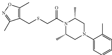
1-(2,6-Dimethyl-4-(o-tolyl)piperazin-1-yl)-2-(((3,5-dimethylisoxazol-4-yl)methyl)thio)ethanone (5k)
