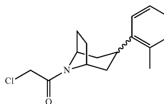
2-Chloro-1-(3-(o-tolyl)-8-azabicyclo[3.2.1]octan-8-yl)ethan-1-one (24)
