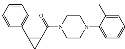
(2-Phenylcyclopropyl)(4-(o-tolyl)piperazin-1-yl) methanone (15)
