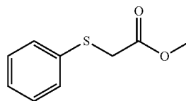
Methyl 2-(phenylthio)acetate (28)
