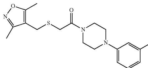
2-(((3,5-Dimethylisoxazol-4-yl)methyl)thio)-1-(4-(m-tolyl)piperazin-1-yl)ethanone (5c)
