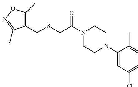
1-(4-(5-Chloro-2-methylphenyl)piperazin-1-yl)-2-(((3,5-dimethylisoxazol-4-yl)methyl)thio)ethan-1-one (BRE454-58)
