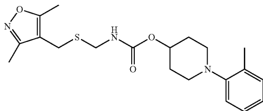
1-(o-Tolyl)piperidin-4-yl(((3,5-dimethylisoxazol-4-yl)methyl)thio)methyl-carbamate (20b)
