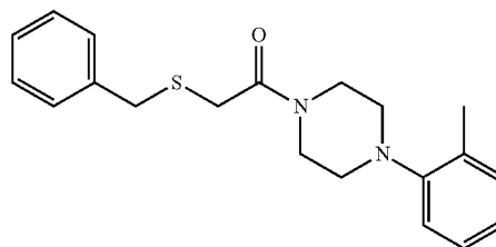
2-(Benzylthio)-1-(4-(o-tolyl)piperazin-1-yl)ethanone (7)
