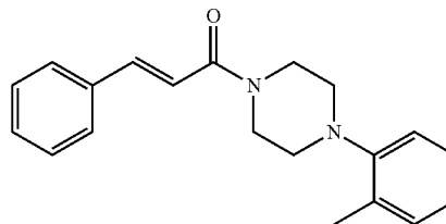
(E)-3-Phenyl-1-(4-(o-tolyl)piperazin-1-yl)prop-2-en-1-one (11)
