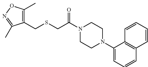
2-(((3,5-Dimethylisoxazol-4-yl)methyl)thio)-1-(4-(naphthalen-1-yl)piperazin-1-yl)ethanone (5g)
