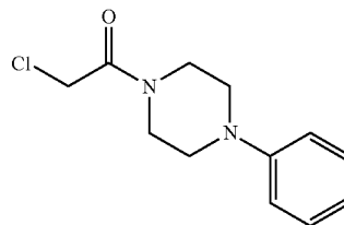
2-Chloro-1-(4-(o-tolyl)piperazin-1-yl)ethanone (17a)
