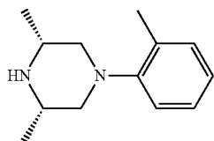
(3S,5R)-3,5-Dimethyl-1-(o-tolyl)piperazine (4k)
