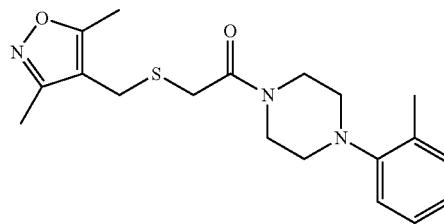
2-(((3,5-Dimethylisoxazol-4-yl)methyl)thio)-1-(4-(o-tolyl)piperazin-1-yl)ethanone (5b)
