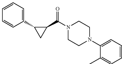
((1S,2S)-2-Phenylcyclopropyl)(4-(o-tolyl)piperazin-1-yl)methanone (16)
