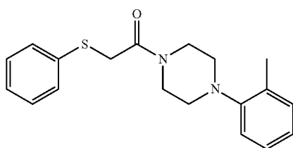
2-(Phenylthio)-1-(4-(o-tolyl)piperazin-1-yl)ethan-1-one (9)
