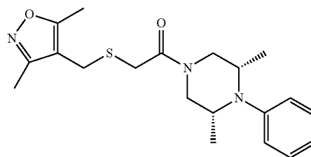
1-(3,5-Dimethyl-4-phenylpiperazin-1-yl)-2-(((3,5-dimethylisoxazol-4-yl)methyl)thio)ethanone (5l)
