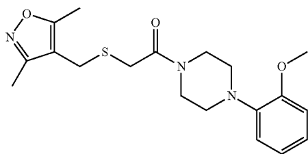
2-(((3,5-Dimethylisoxazol-4-yl)methyl)thio)-1-(4-(2-methoxyphenyl)piperazin-1-yl)ethanone (5h)
